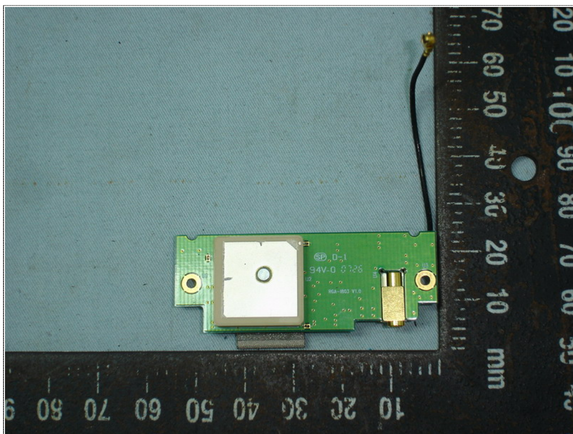
Front View of GPS
