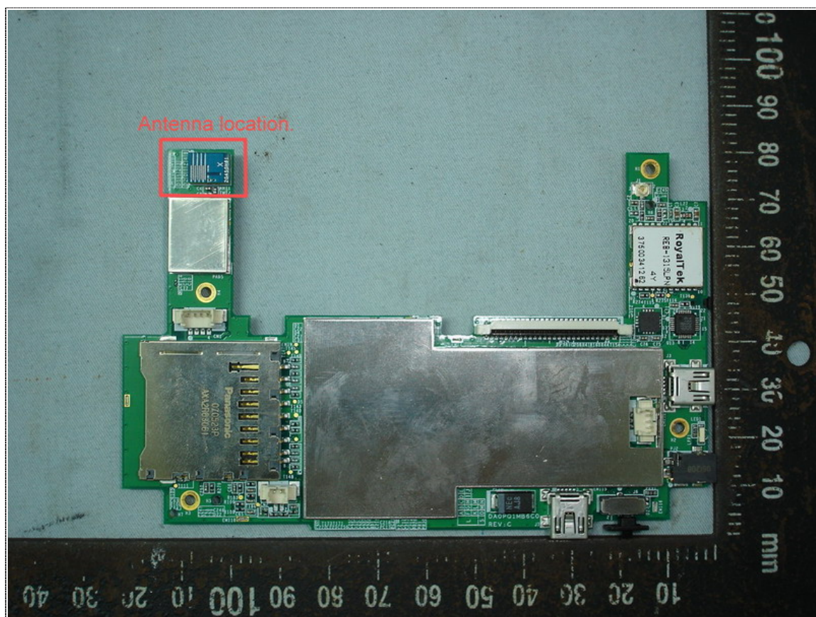
Antenna Location
