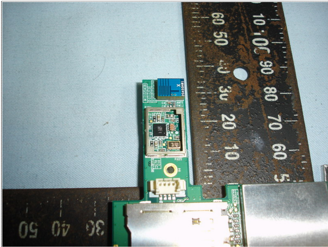
Component View of Bluetooth Board
