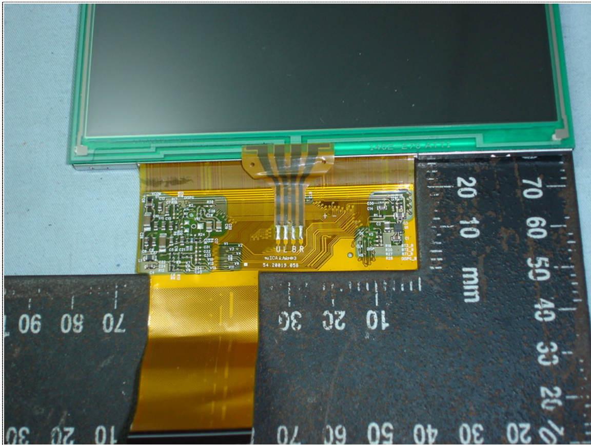
Component View of Panel Control Board
