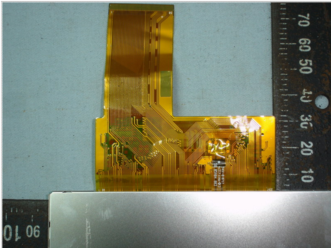
Solder View of Panel Control Board
