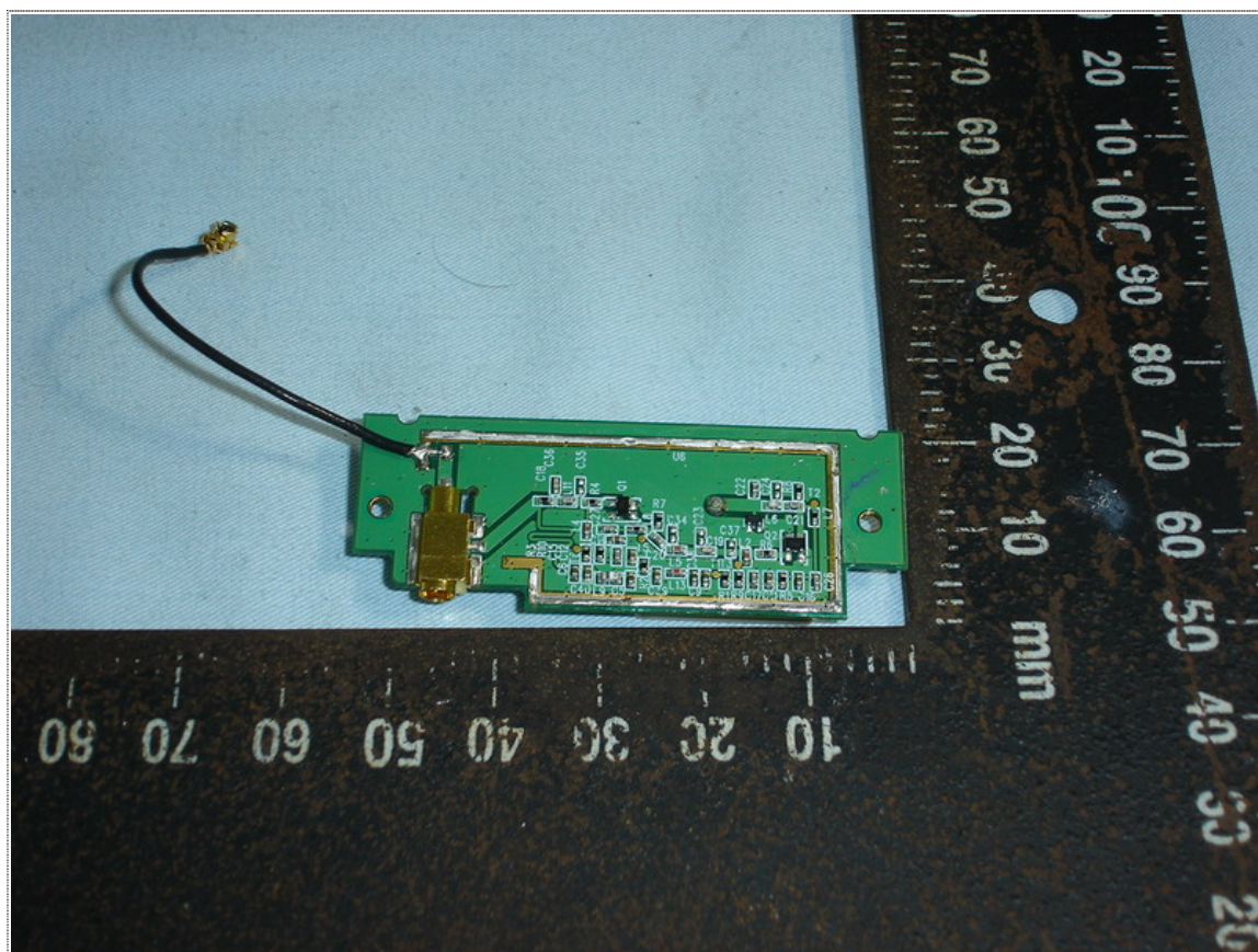
Rear View of GPS
