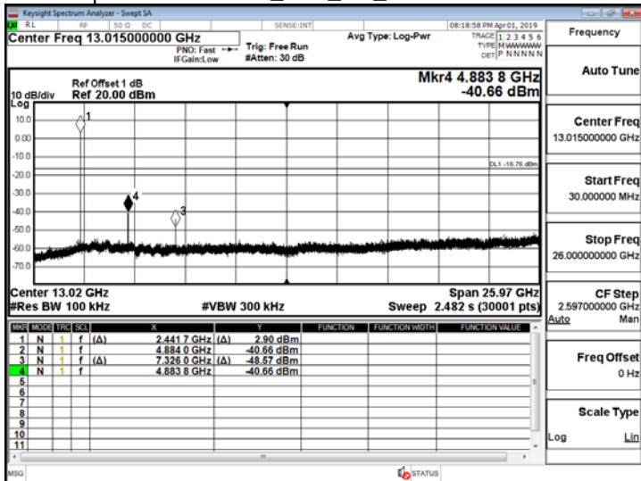
Spurious Emission_BLE_1M_MidCH19-2442
