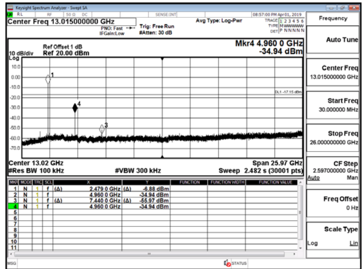
Spurious Emission_BLE_2M_HighCH39-2480
