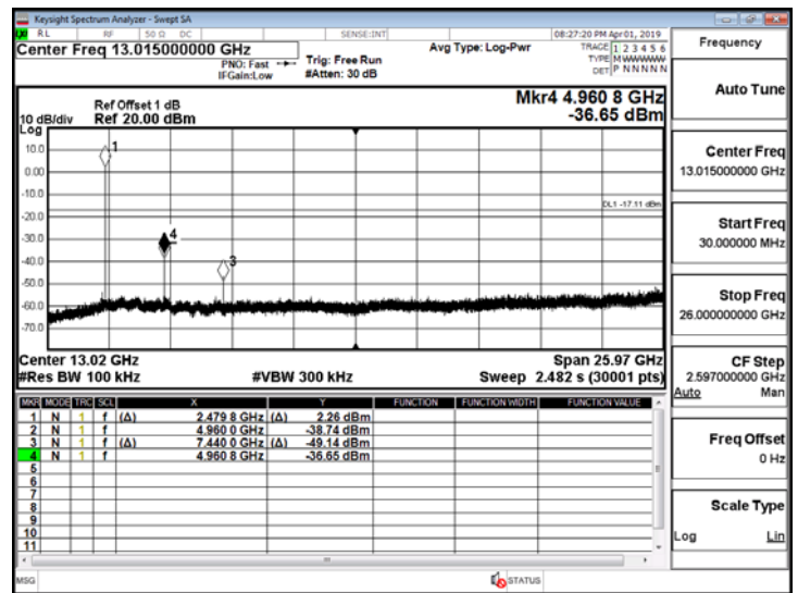
Spurious Emission_BLE_1M_HighCH39-2480
