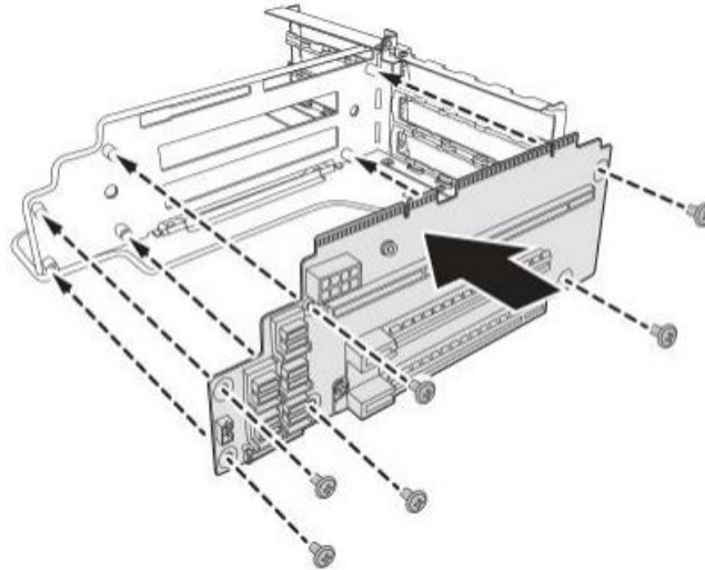
Figure 1-41: Installing the Riser 1 Board
