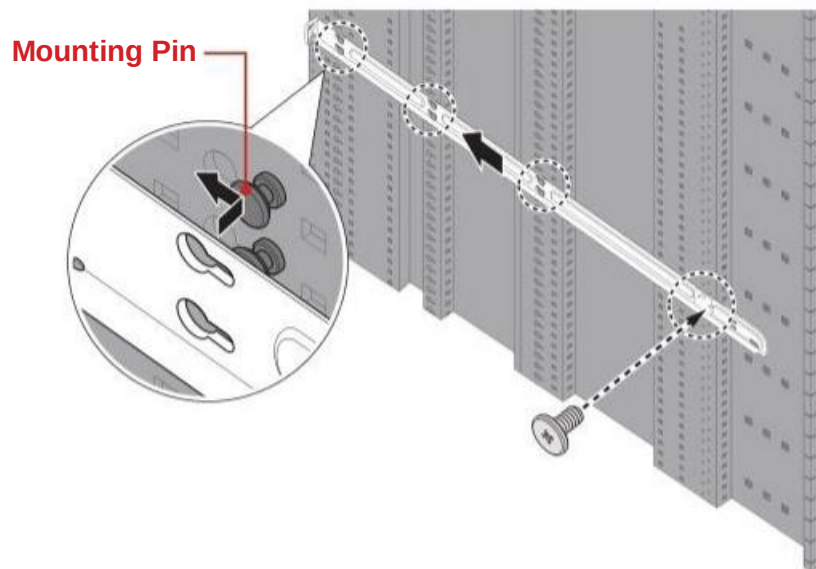
Figure 2-2: Installing the Right Rail
