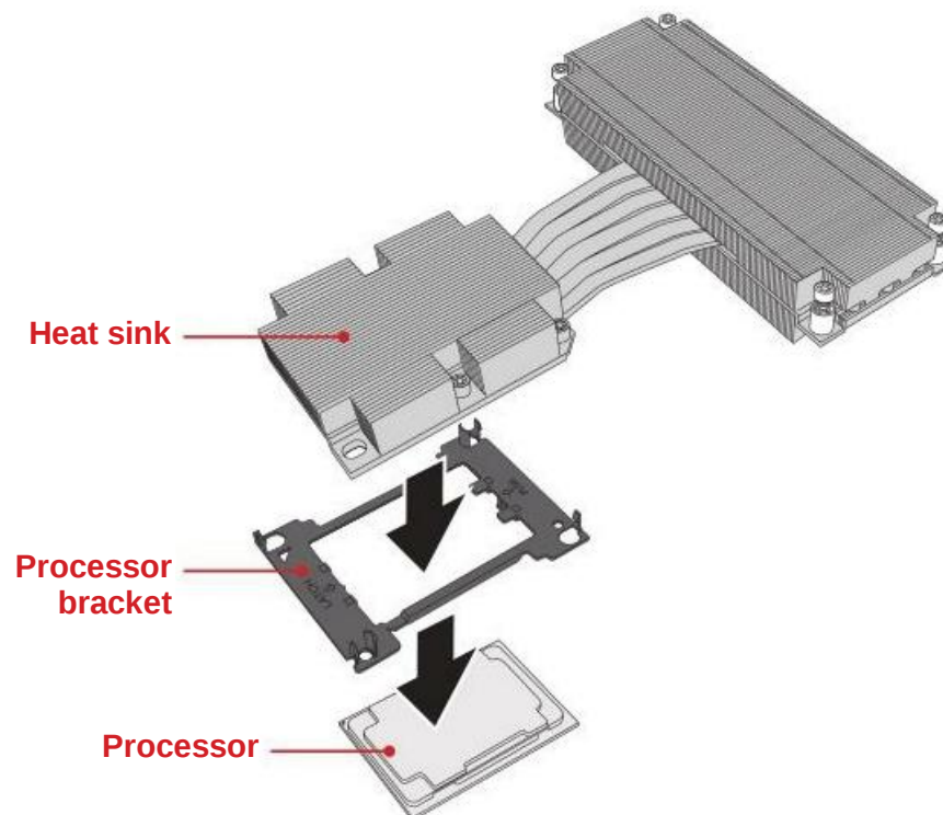
Figure 1-58: Removing the Processor
