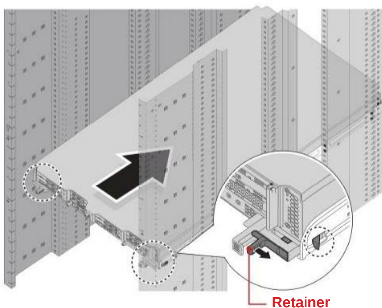
Figure 2-3: Installing the Server in the Rack
