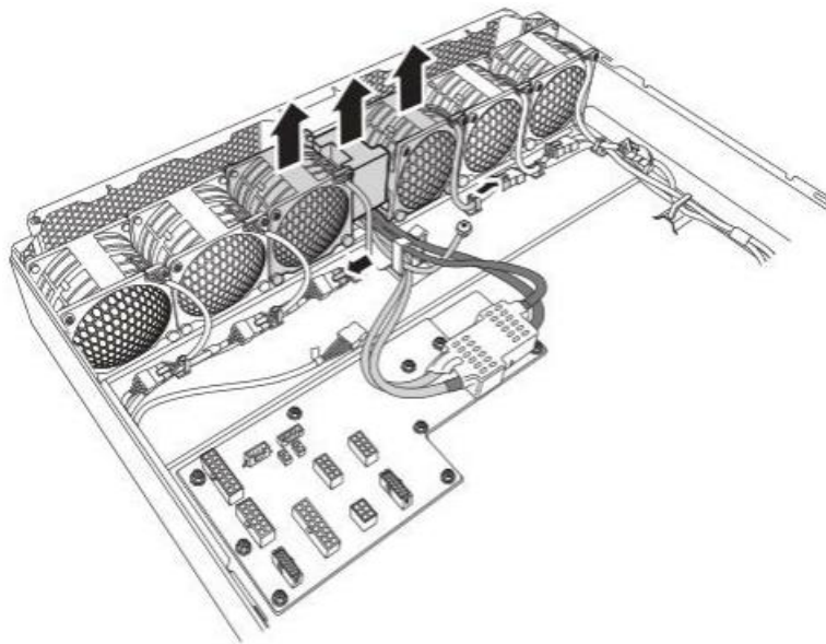
Figure 1-14: Removing the Fan Modules and Rubber Pad
