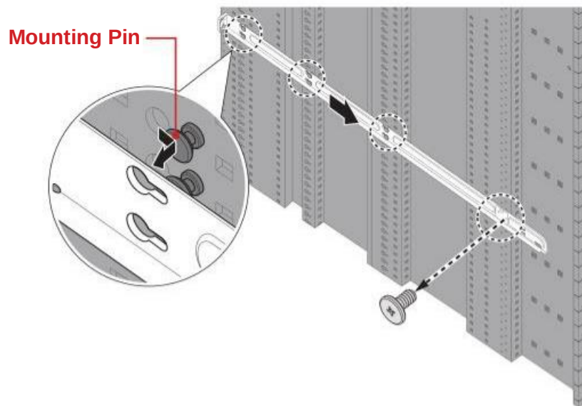
Figure 2-5: Removing the Right Rail
