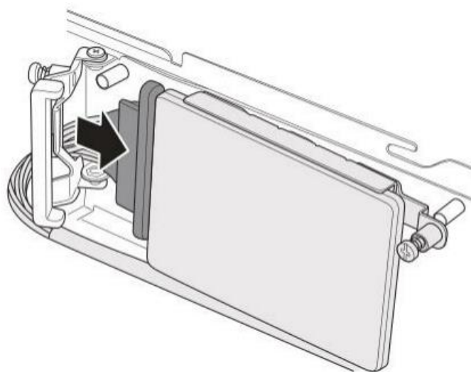
Figure 1-29: Connecting the Oculink Cable
