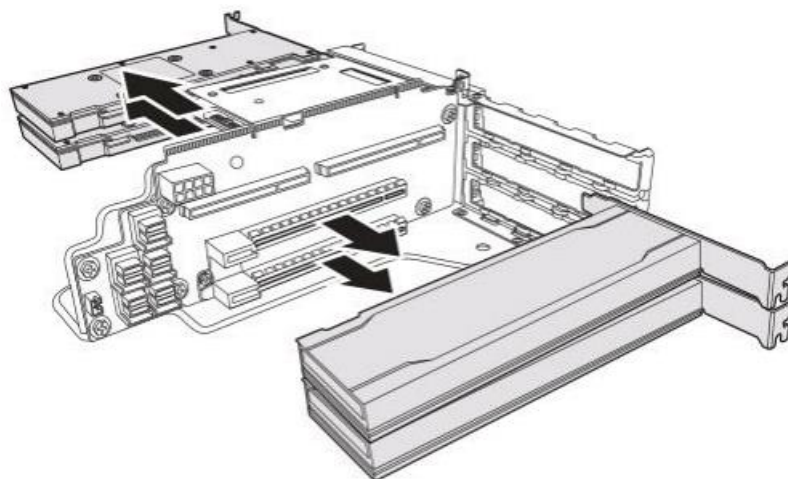
Figure 1-45: Removing the Tesla T4 Cards
