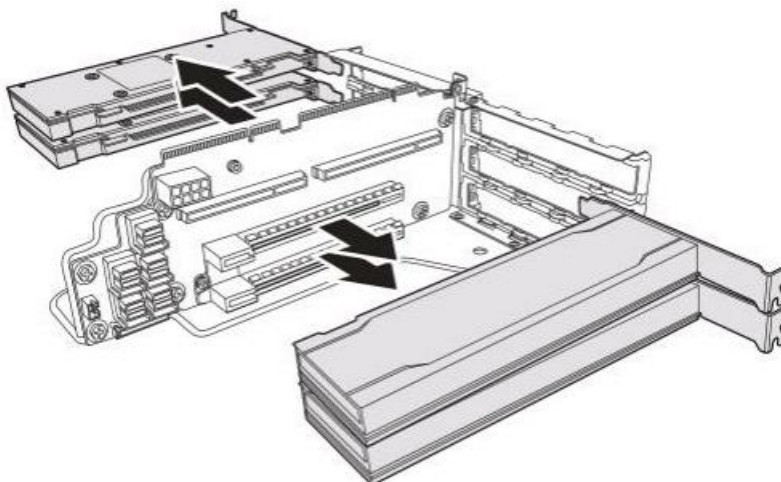
Figure 1-35: Removing the Tesla T4 Cards
