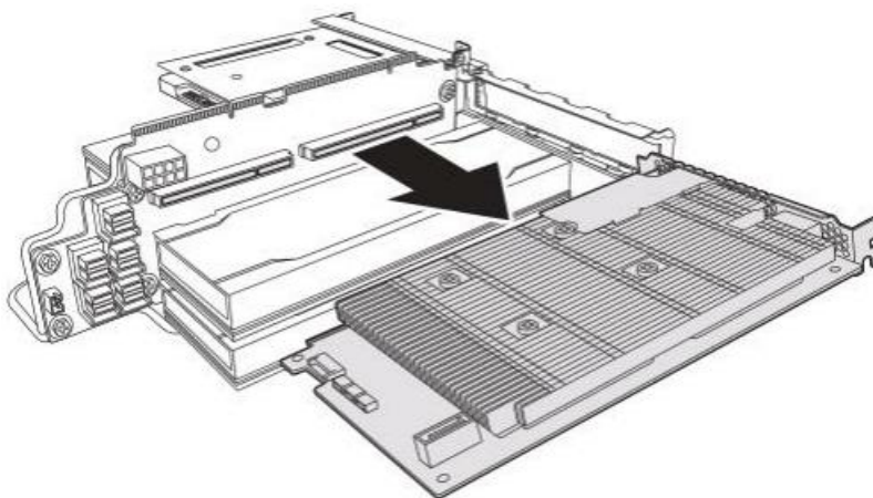
Figure 1-44: Removing the K2X-N Card
