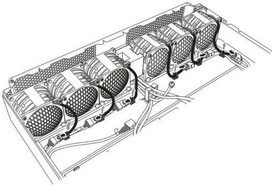
Figure 1-8: Disconnecting the Fan Cables
