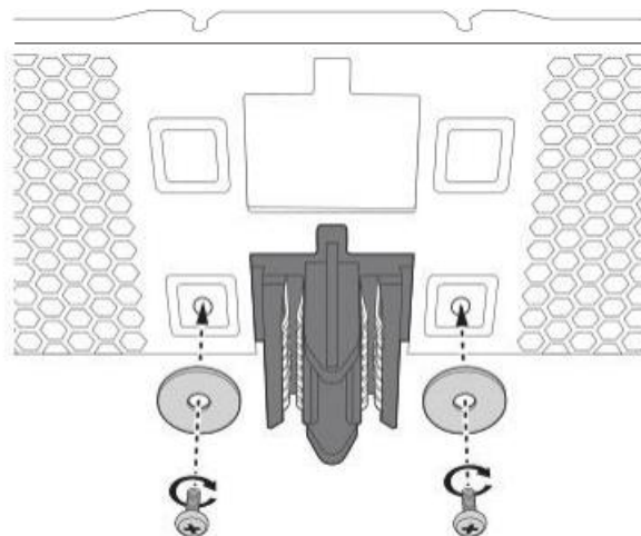
Figure 1-21: Installing the the Screws and Washers
