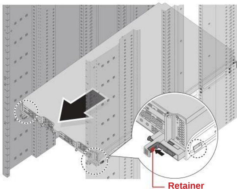
Figure 2-4: Removing the Server
