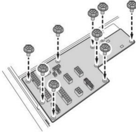
Figure 1-19: Installing the PDB Board
