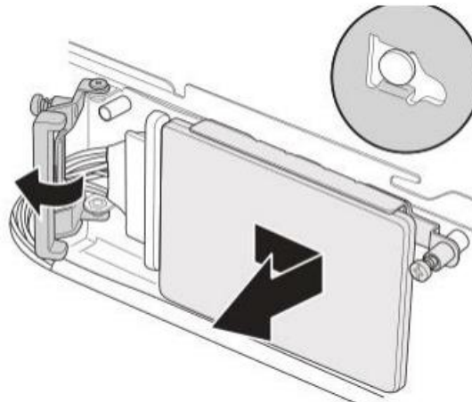
Figure 1-25: Removing the NVMe SSD Assembly
