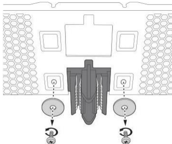
Figure 1-16: Removing the Screws and Washers
