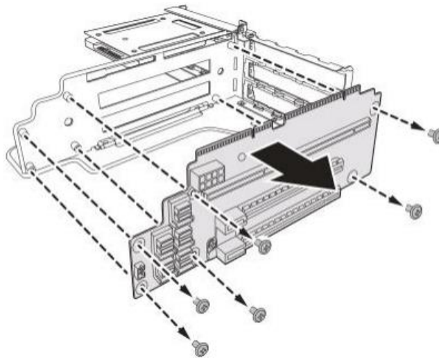
Figure 1-50: Removing the Riser 2 Board
