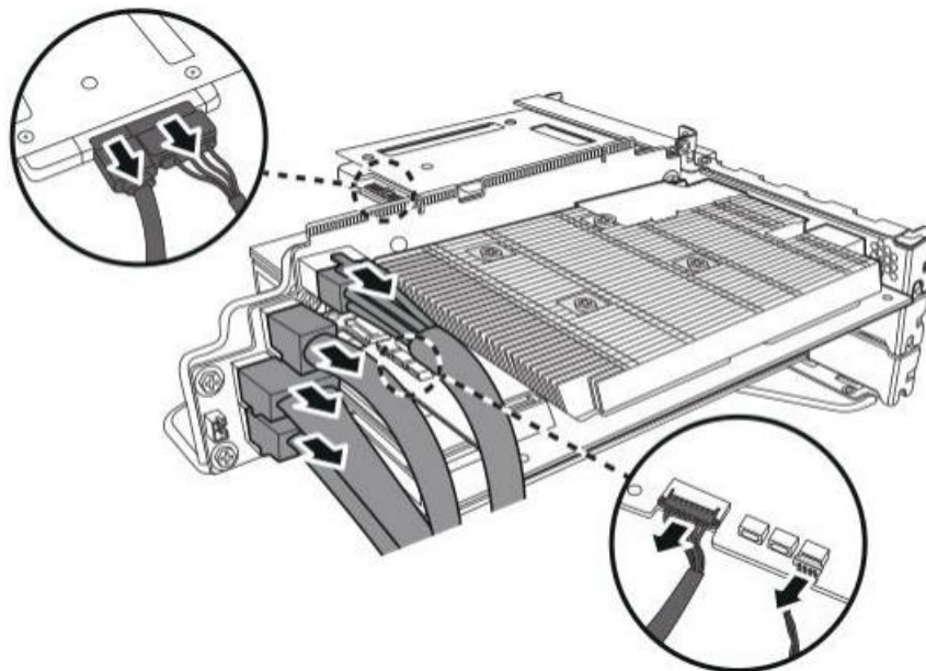
Figure 1-43: Disconnecting the Cables
