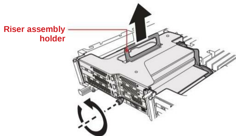
Figure 1-42: Removing the Riser 2 Assembly
