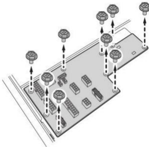
Figure 1-18: Removing the PDB Board
