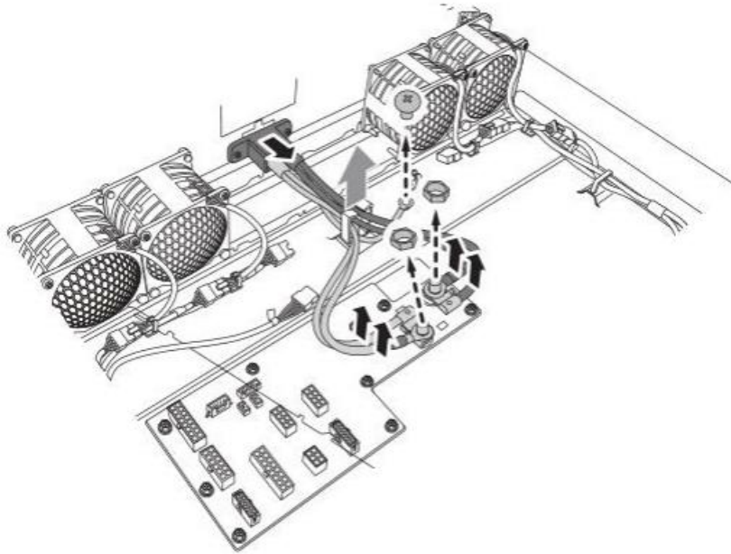
Figure 1-17: Removing the Busbar Power Cables
