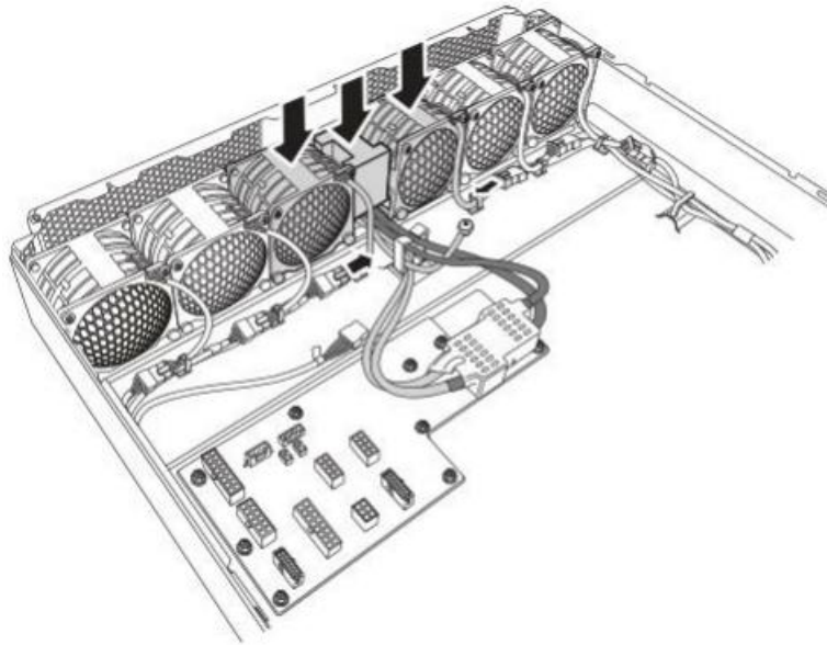
Figure 1-23: Installing the Fan Modules and Rubber Pad
