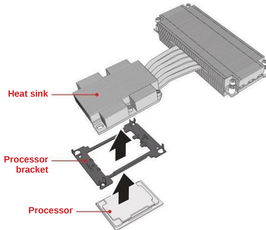
Figure 1-59: Installing the Processor
