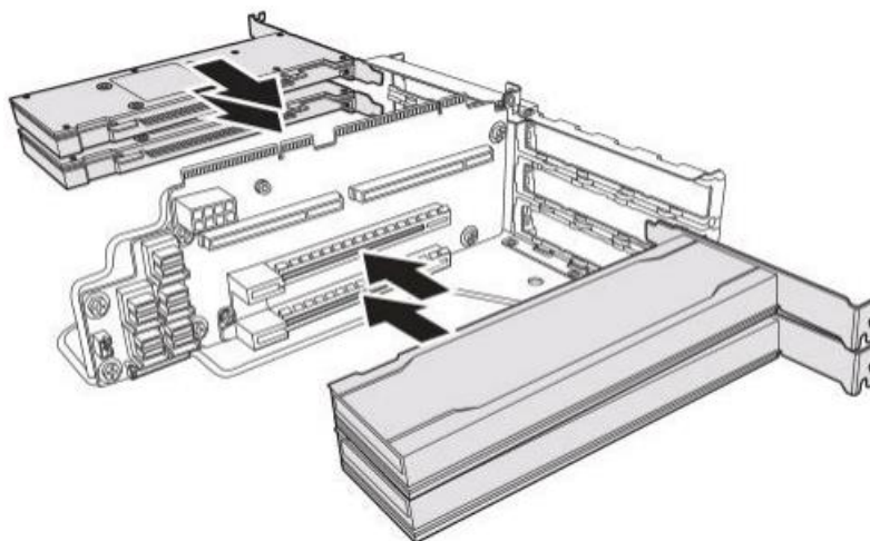
Figure 1-36: Installing the Tesla T4 Cards
