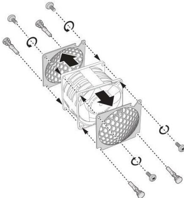
Figure 1-11: Installing the Fan Cages
