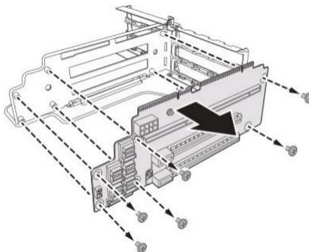
Figure 1-40: Removing the Riser 1 Board
