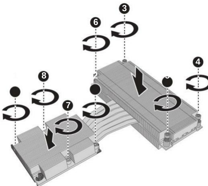
Figure 1-57: Installing the Heat Sink
