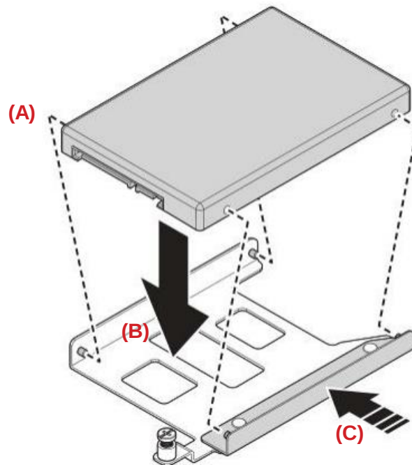
Figure 1-28: Installing the NVMe SSD
