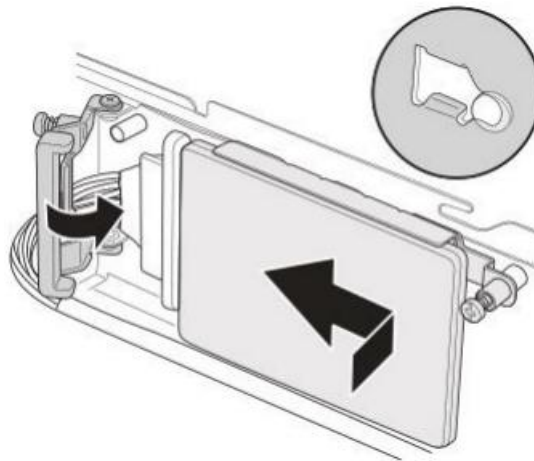
Figure 1-30: Installing the NVMe SSD Assembly
