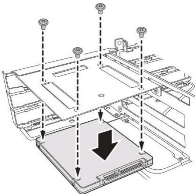
Figure 1-55: Installing the SATA SSD
