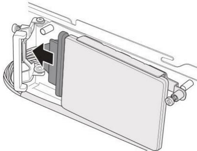
Figure 1-26: Disconnecting the Oculink Cable
