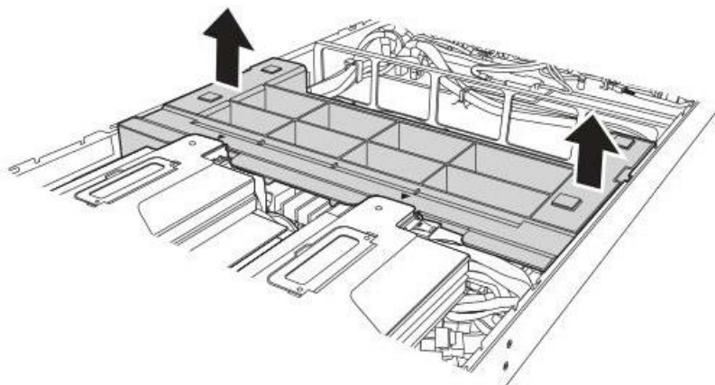
Figure 1-6: Removing the Air Duct
