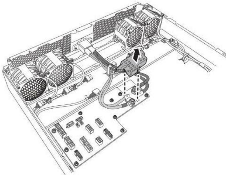
Figure 1-15: Removing the Cable Protective Cap
