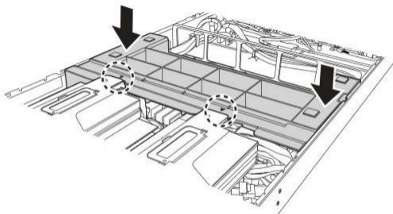
Figure 1-7: Installing the Air Duct
