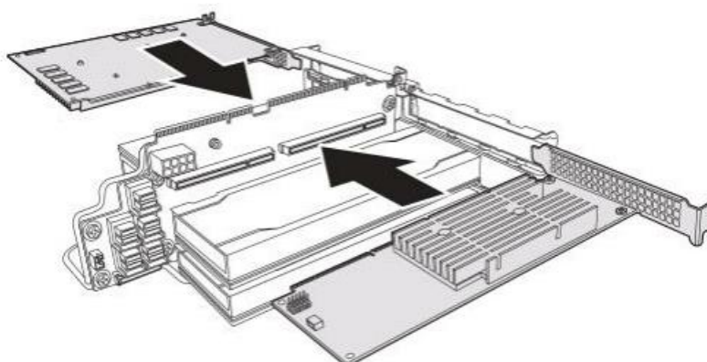
Figure 1-37: Installing the K2T-QB and K2C-AB Cards
