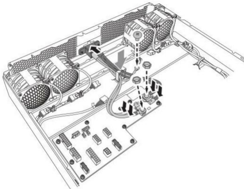
Figure 1-20: Installing the Busbar Power Cables
