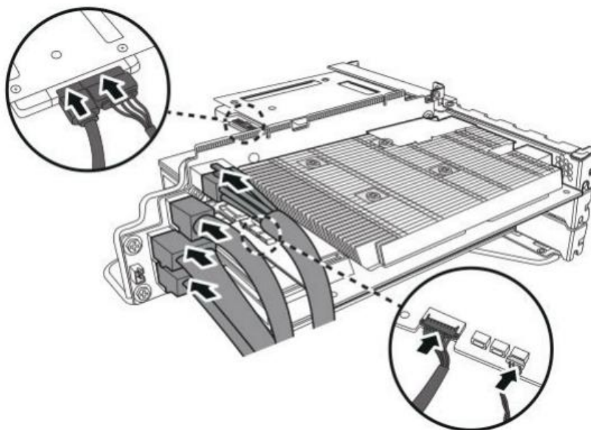
Figure 1-48: Connecting the Cables
