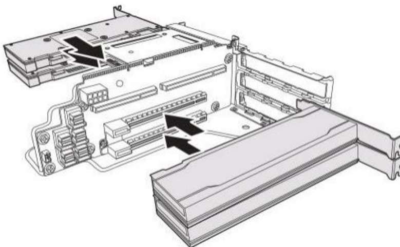
Figure 1-46: Installing the Tesla T4 Cards
