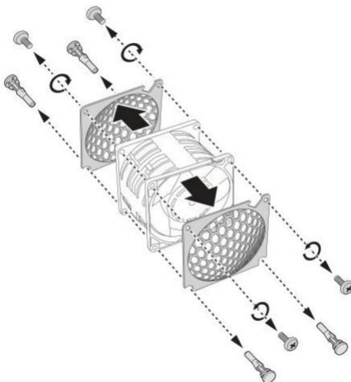
Figure 1-10: Removing the Fan Cages
