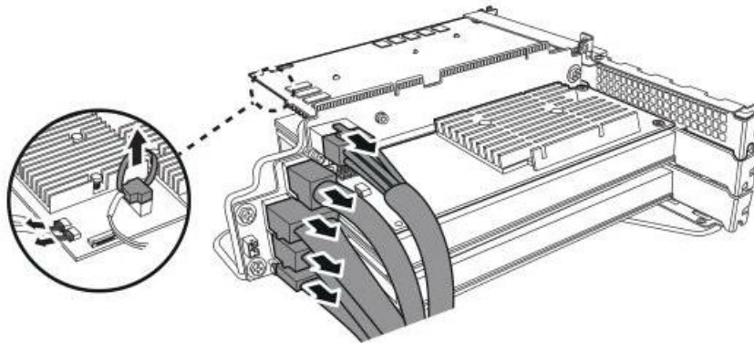
Figure 1-33: Disconnecting the Cables
