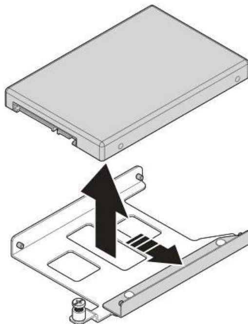
Figure 1-27: Removing the NVMe SSD
