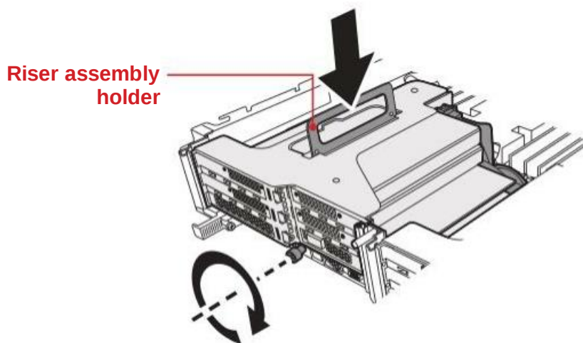
Figure 1-49: Installing the Riser 2 Assembly
