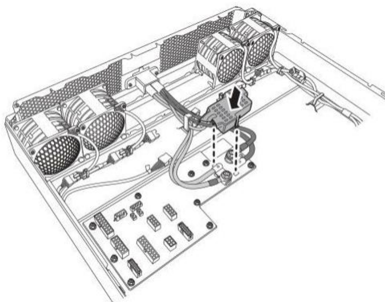
Figure 1-22: Installing the Cable Protective Cap
