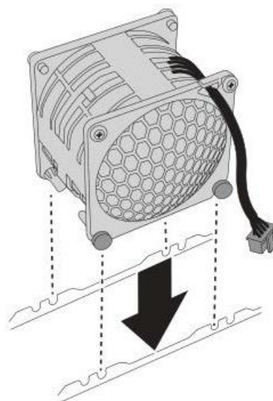
Figure 1-12: Installing the Fan Module Assembly
