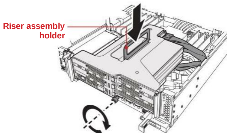
Figure 1-39: Installing the Riser 1 Assembly
