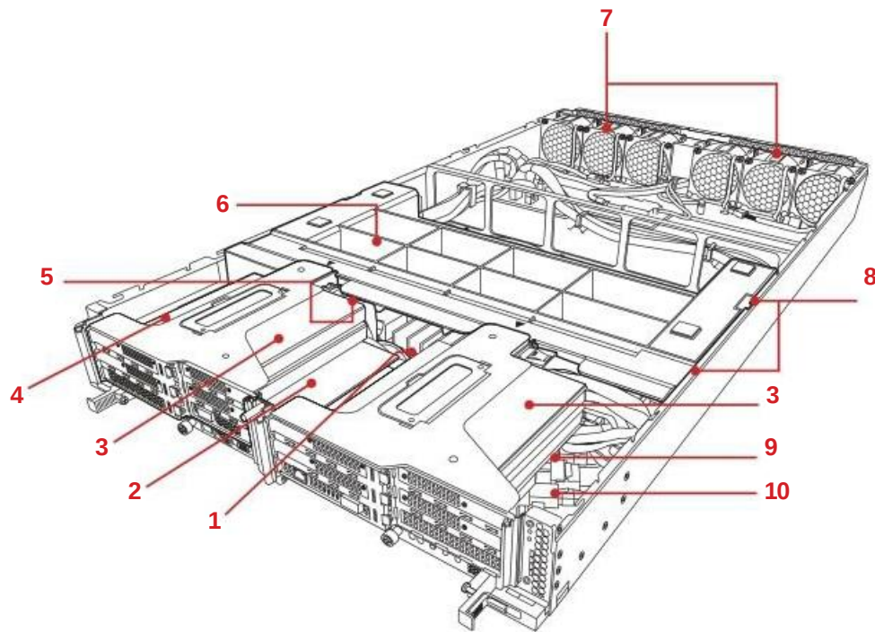
Figure 1-1: Component View
