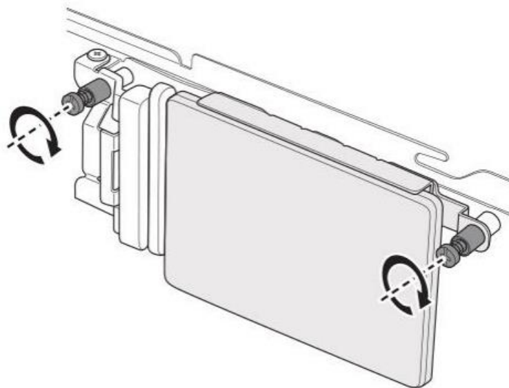
Figure 1-31: Tightening the Screws
