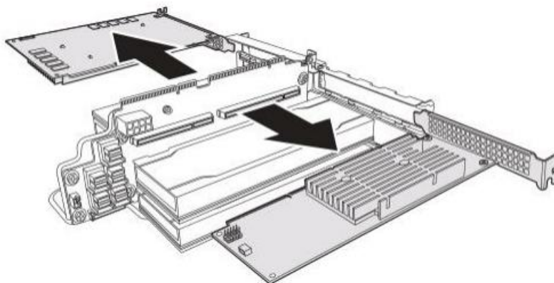
Figure 1-34: Removing the K2T-QB and K2C-AB Cards
