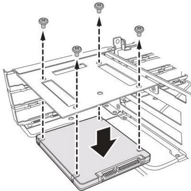
Figure 1-52: Removing the SATA SSD
