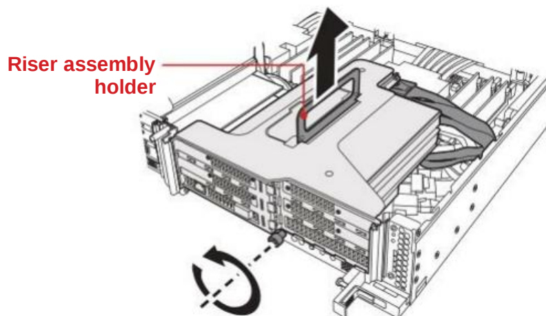
Figure 1-32: Removing the Riser 1 Assembly
