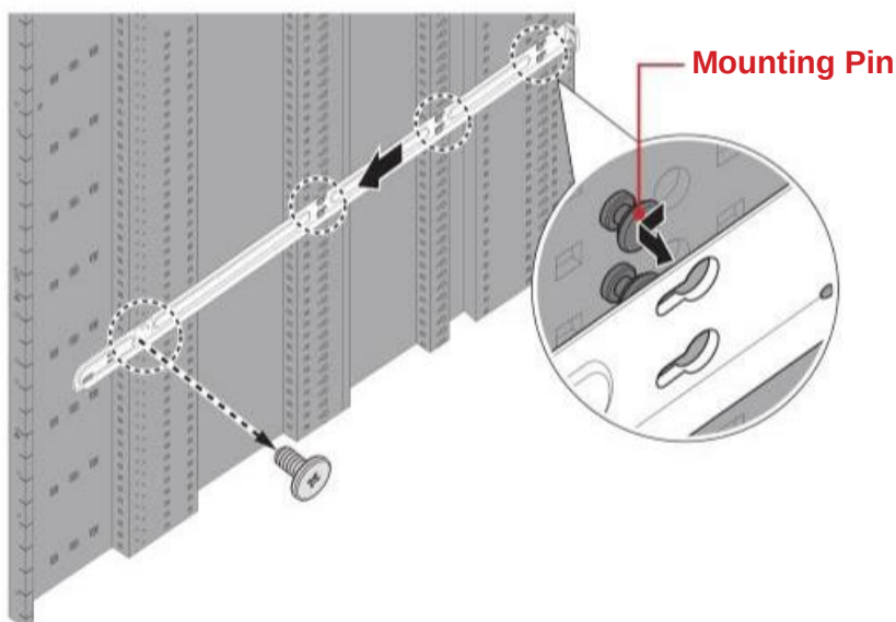
Figure 2-6: Removing the Left Rail
