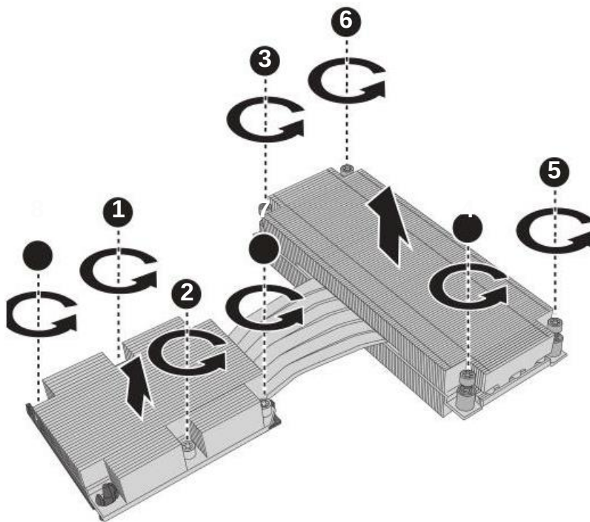
Figure 1-56: Removing the Heat Sink
