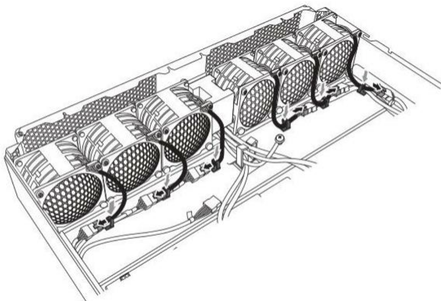
Figure 1-13: Connecting the Fan Cables
