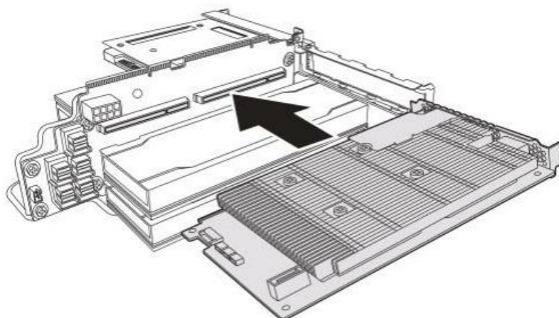
Figure 1-47: Installing the K2X-N Card
