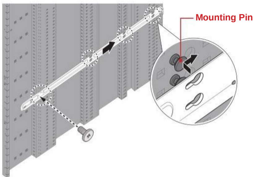
Figure 2-1: Installing the Left Rail
