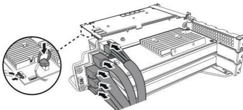
Figure 1-38: Connecting the Cables
