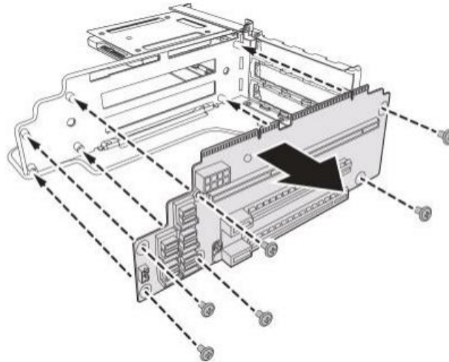
Figure 1-51: Installing the Riser 2 Board
