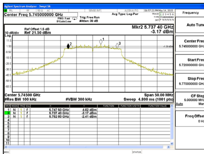
Figure Channel 149:
