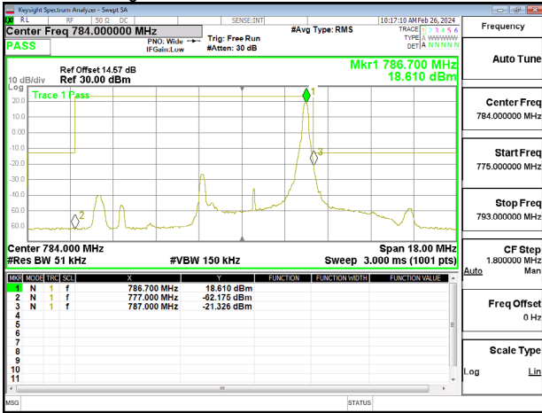
Band Edge_Band13_5MHz_QPSK_RB25_0_CH23205
