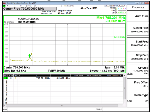
Band13_5MHz_QPSK_RB25_0_CH23205
