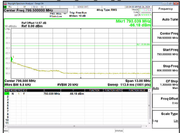
Band13_5MHz_QPSK_RB25_0_CH23255
