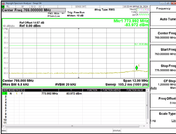
Band13_5MHz_QPSK_RB1_0_CH23205
