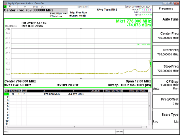
Band13_5MHz_QPSK_RB1_24_CH23255
