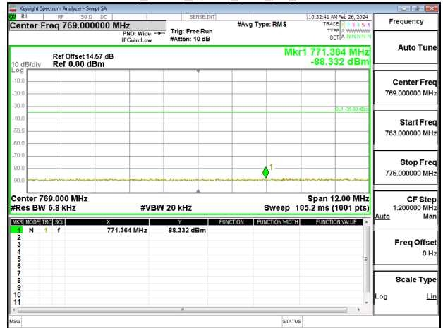
Band13_5MHz_QPSK_RB1_24_CH23255
