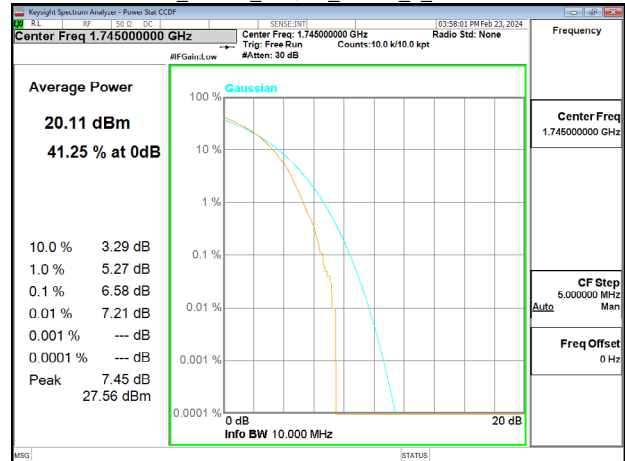
Band4 20MHz 16QAM_RB100_0_CH20300
