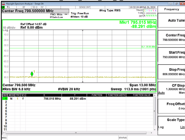
Band13_5MHz_QPSK_RB1_0_CH23205
