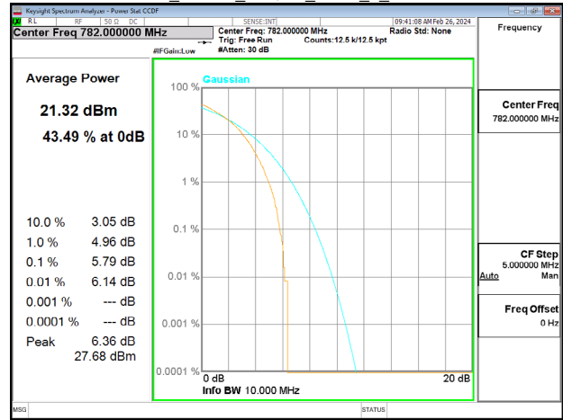
Band13_10MHz_16QAM_RB50_0_CH23230
