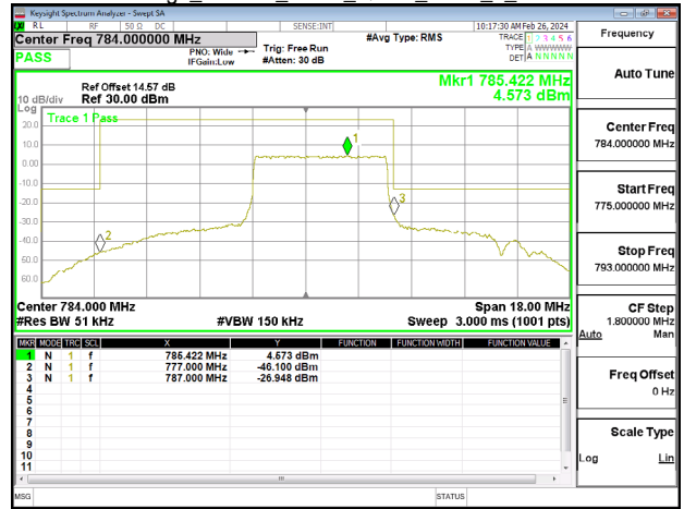
Band13_5MHz_QPSK_RB1_0_CH23205
