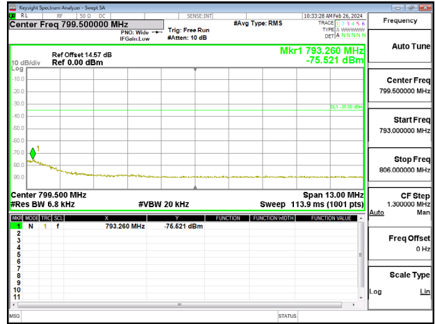
Band13_5MHz_QPSK_RB25_0_CH23255
