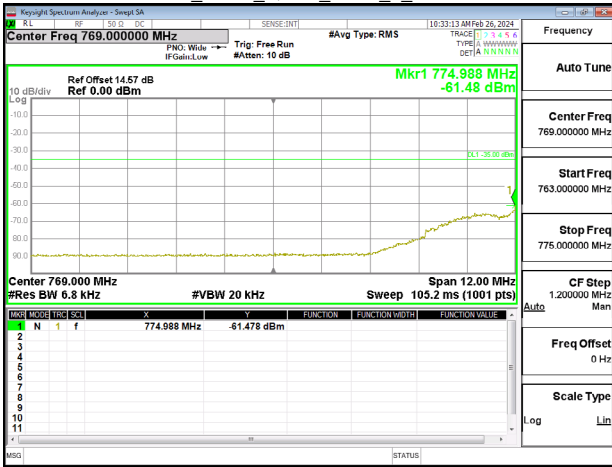
Band13_5MHz_QPSK_RB25_0_CH23255
