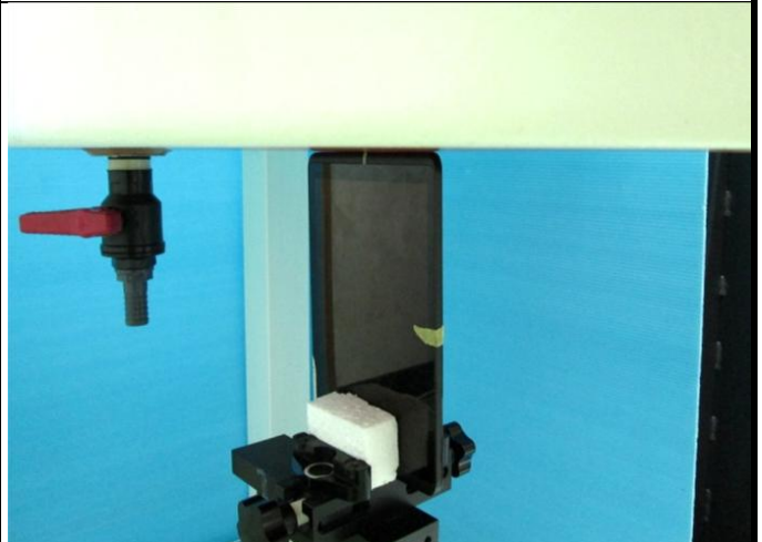
Bottom Side of EUT with 0 mm Gap
