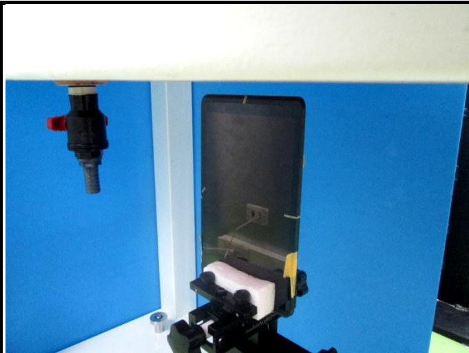
Bottom Side of EUT with 5 mm Gap
