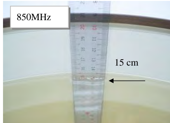
Fig.2.1 Flat
