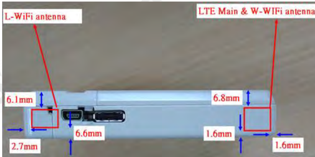
Fig.4 QD8 Antenna location & distance
