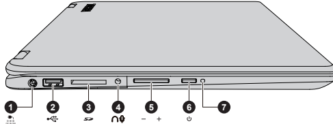
Figure 3-2 The left side of the computer
