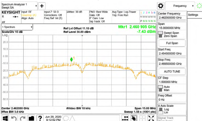
FCC_15_247_WLANPower Density_802.11b_20MHz_Chain0_2462MHz
