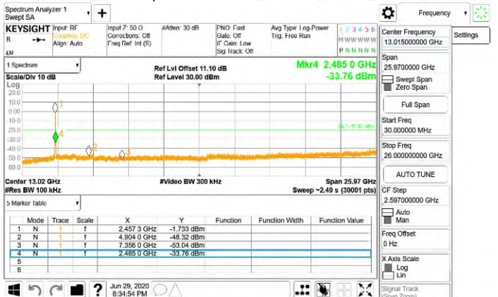
FCC_15_247_WLAN\Spurious Emission_802.11n_40MHz_Chain0_2452MHz
