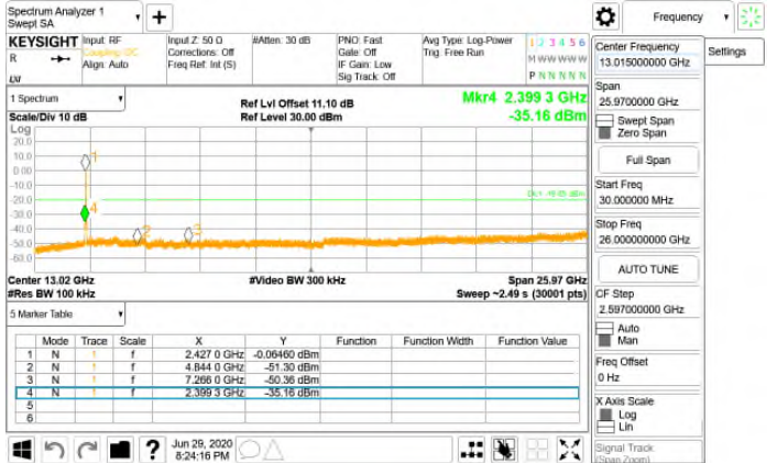
FCC_15_247_WLAN\Spurious Emission_802.11n_40MHz_Chain0_2437MHz
