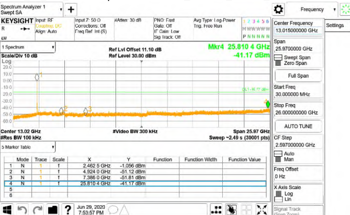
FCC_15_247_WLAN\Spurious Emission_802.11n_20MHz_Chain0_2462MHz
