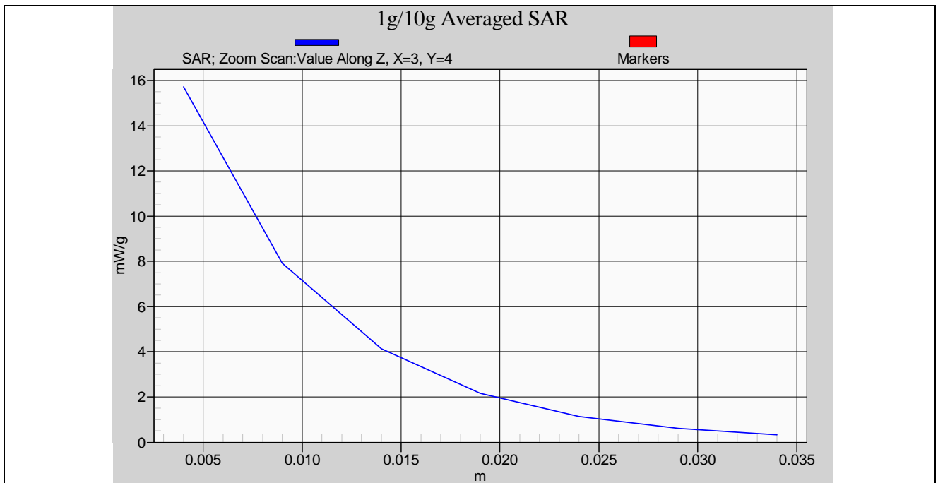
Body-Tissue-Simulating-Liquid 2.4GHz (2008/11/19)
