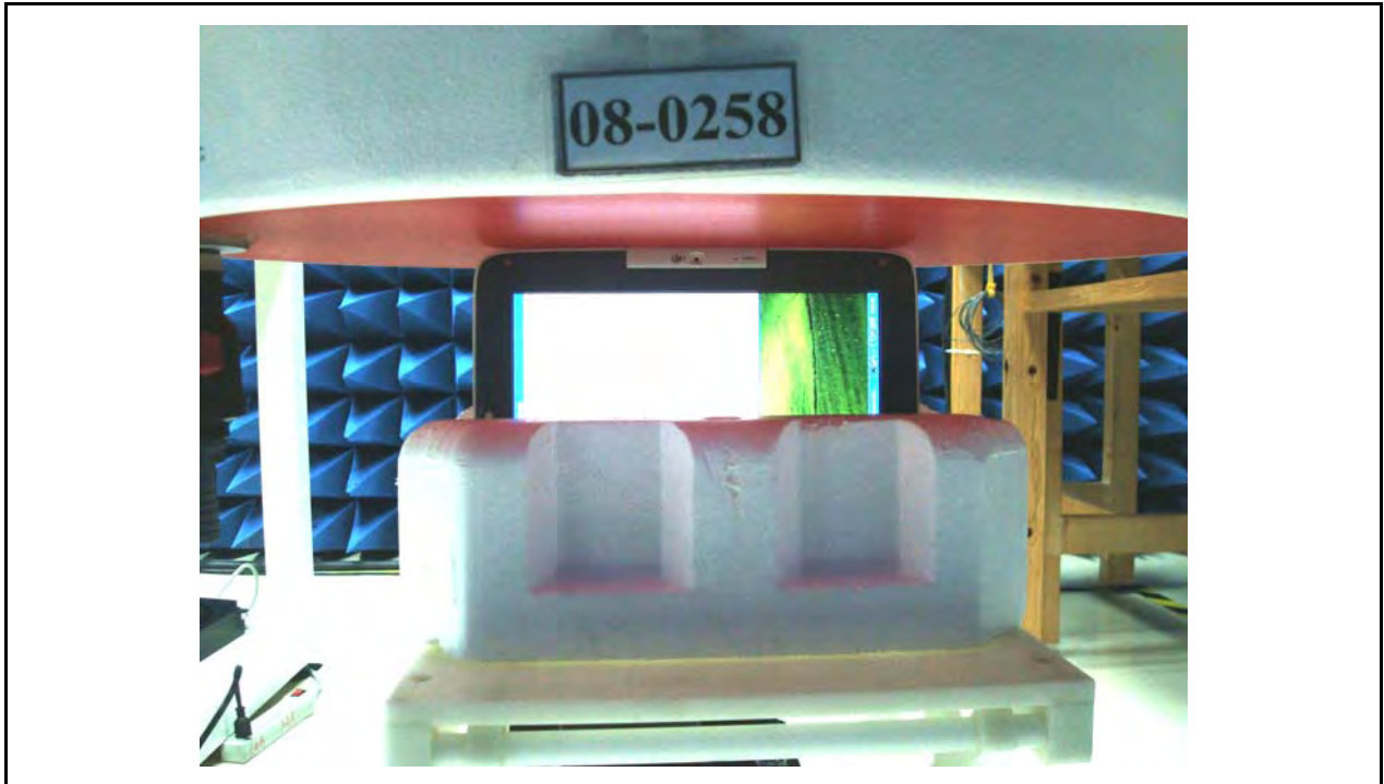
Figure 20. Body SAR Test Setup (Flat Section) _ Tablet Mode EUT Tip to Phantom
