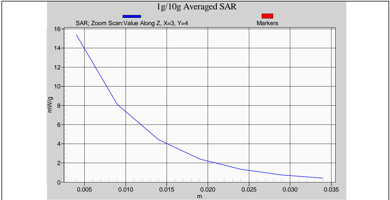
Body-Tissue-Simulating-Liquid 2.4GHz (2008/11/02)
