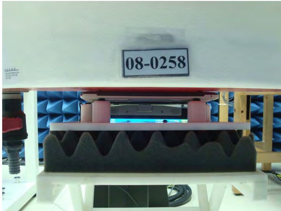
Figure 14. Body SAR Test Setup (Flat Section) _ Normal Mode(LCD open 90° )
