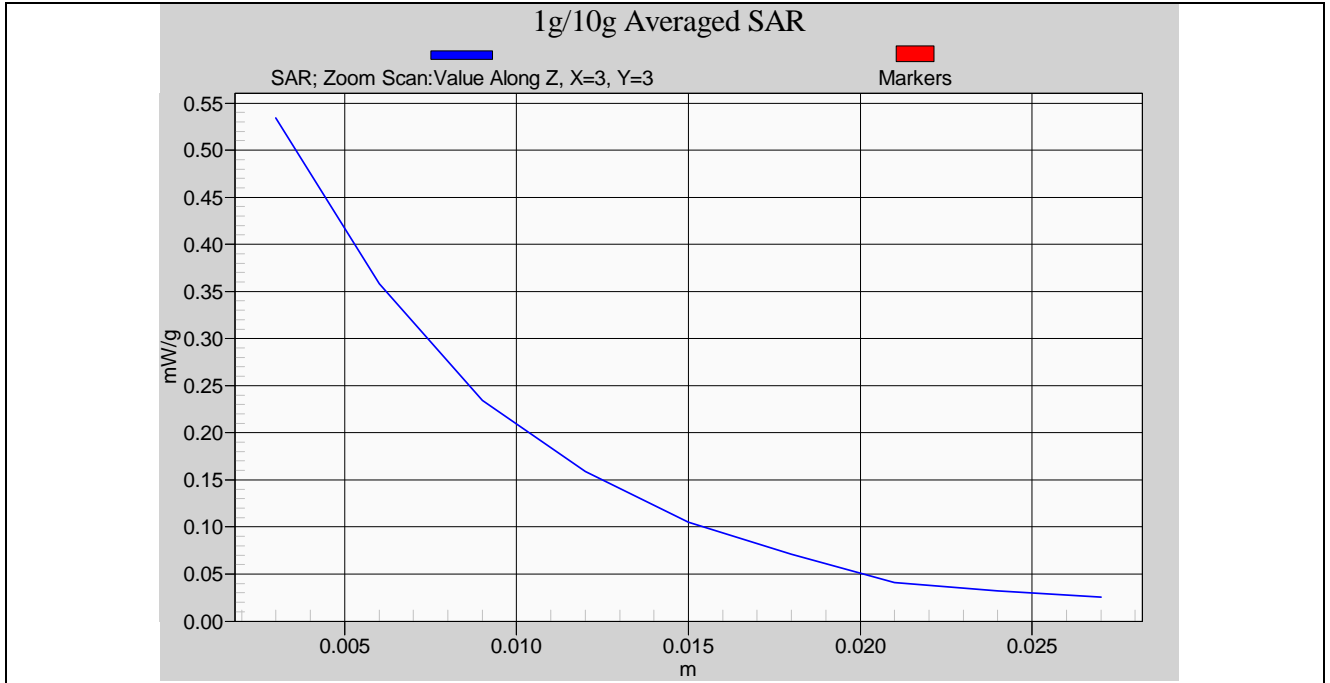
SAR Measurement (Flat Section_ Tablet mode EUT tip to phantom) _ 802.11n HT40 Rate13 CH3
