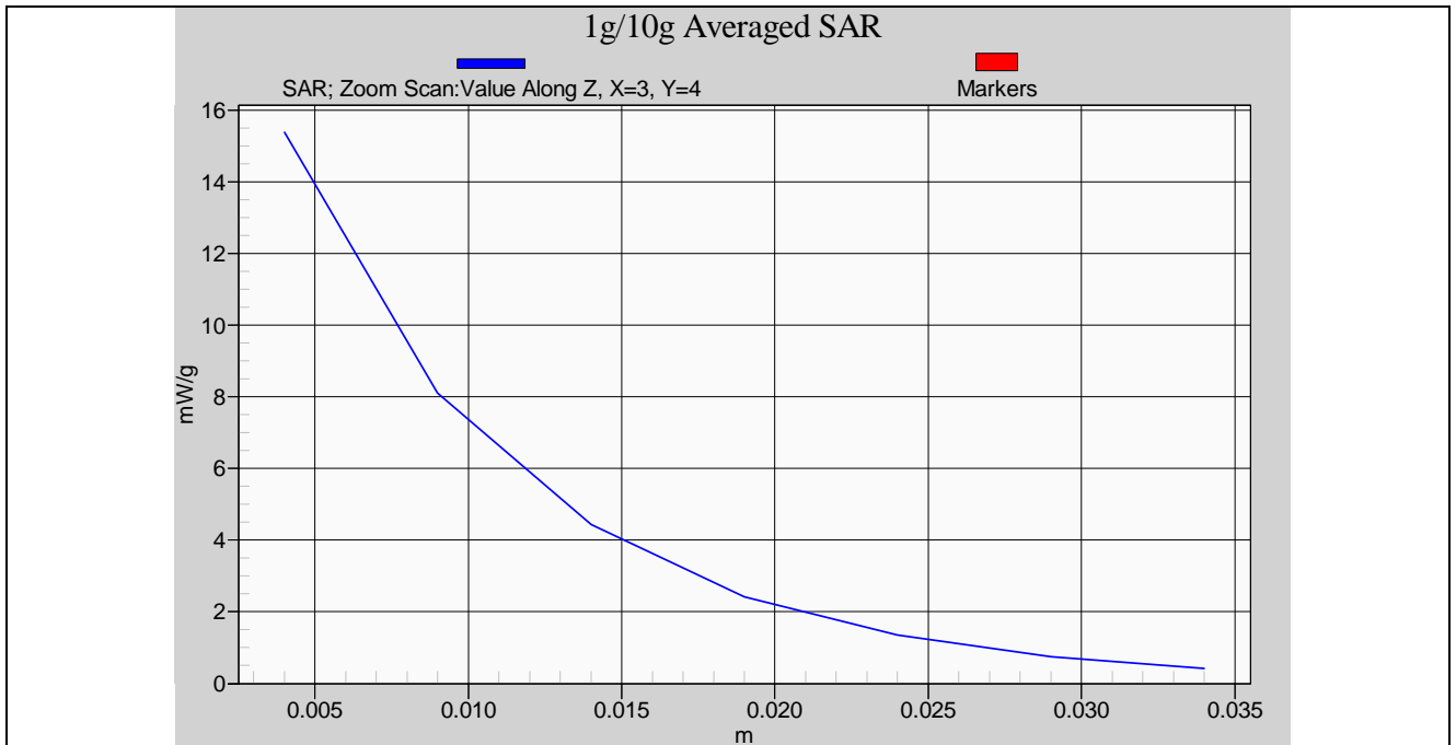
Body-Tissue-Simulating-Liquid 2.4GHz (2008/10/31)
