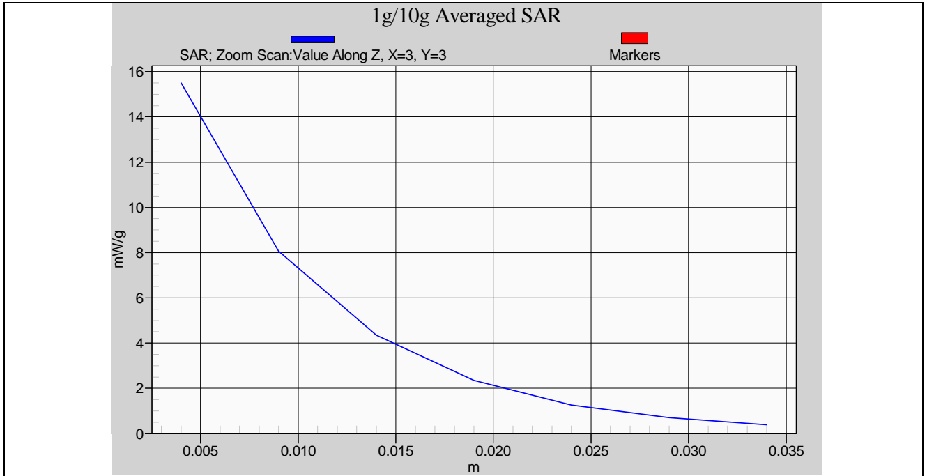
Body-Tissue-Simulating-Liquid 2.4GHz (2008/10/29)
