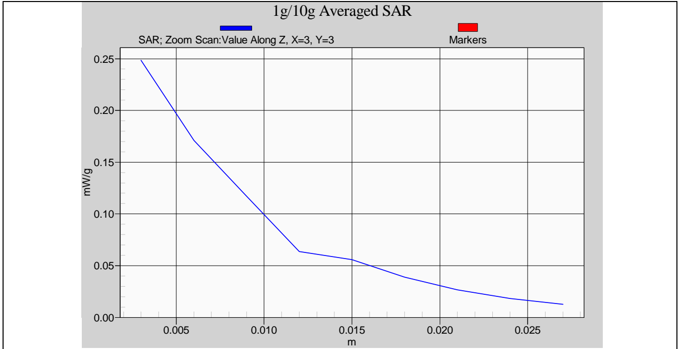
SAR Measurement (Flat Section_ Tablet mode EUT tip to phantom) _ 802.11b Rate11 CH1
