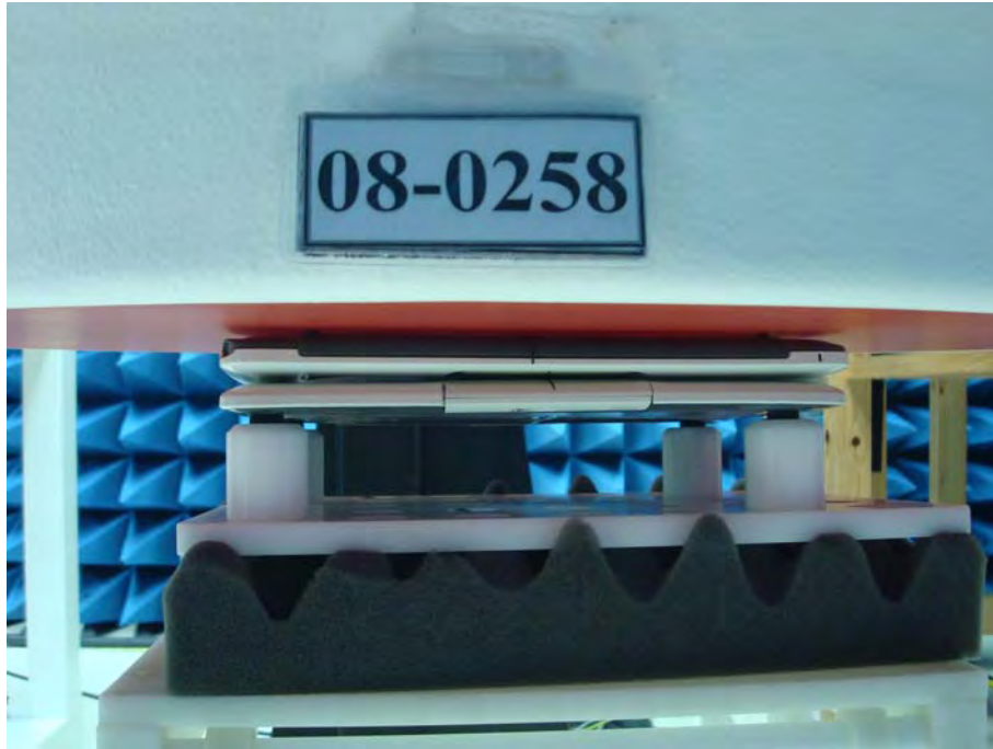
Figure 17. Body SAR Test Setup (Flat Section) _ Tablet Mode EUT Bottom to Phantom
