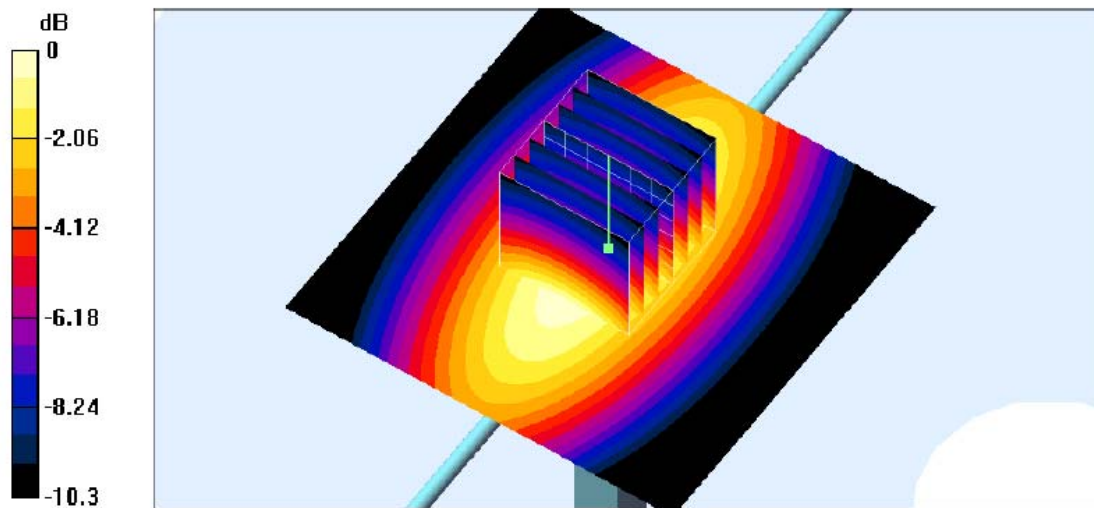
0 dB = 1.04mW/g
