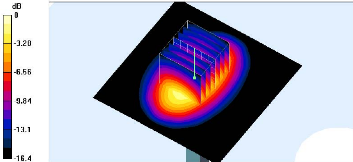
0 dB = 4.62mW/g
