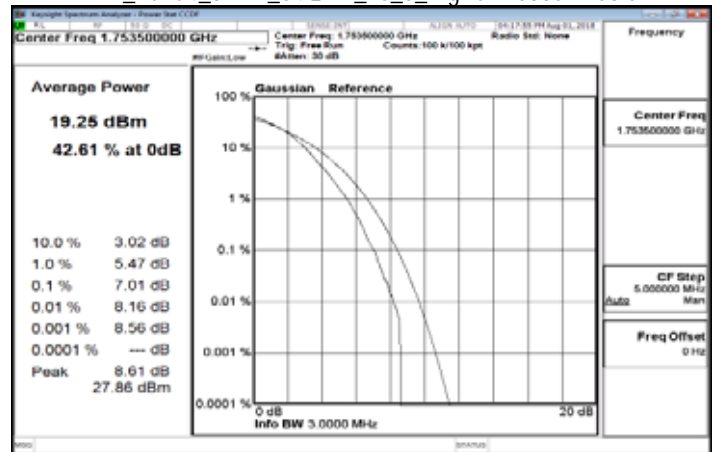
LTE_Band4_3MHz_64QAM_15_0_HighCH20385-1753.5
