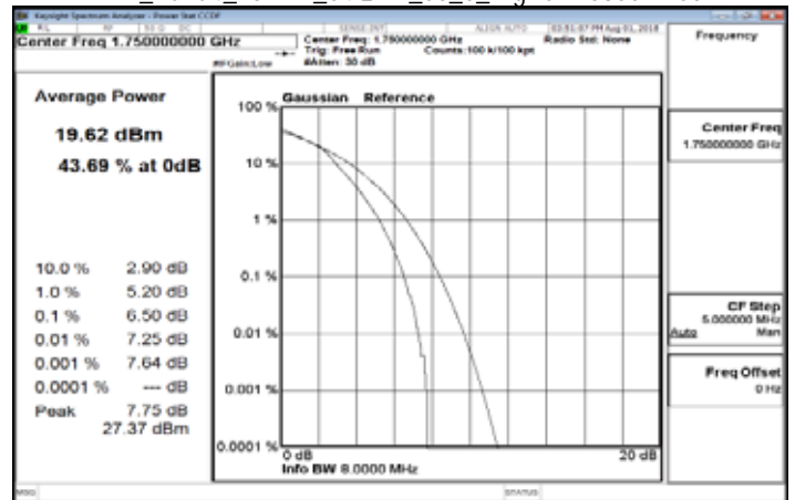
LTE_Band4_10MHz_64QAM_50_0_HighCH20350-1750
