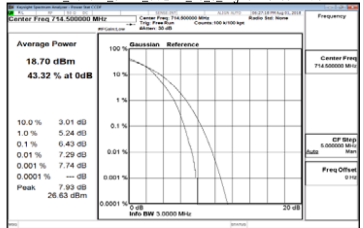
LTE_Band12_3MHz_64QAM_15_0_HighCH23165-714.5
