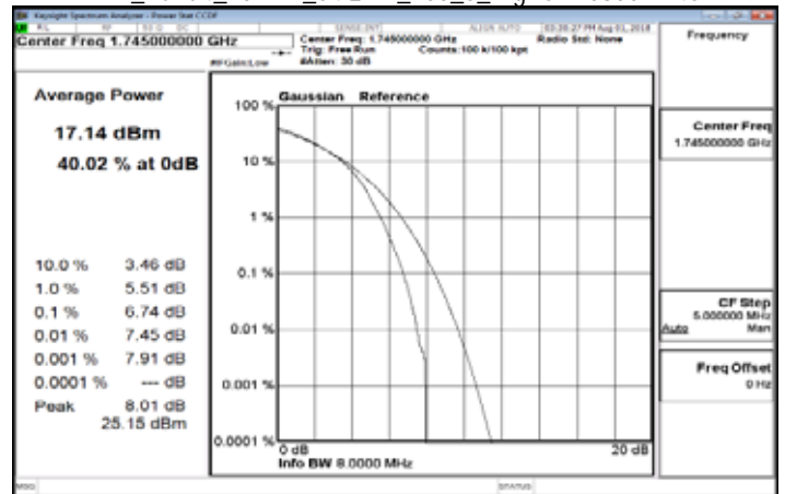
LTE_Band4_20MHz_64QAM_100_0_HighCH20300-1745
