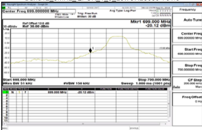
Band12_5MHz_QPSK_1_0_LowCH23035-701.5
