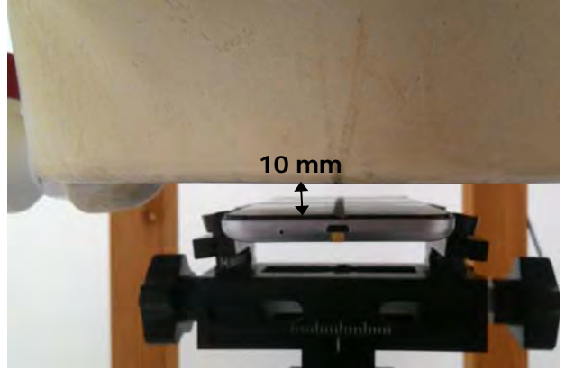
Fig.8 EUT front side to flat phantom
