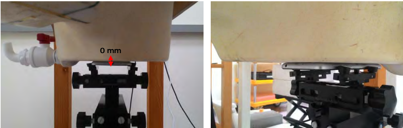
Fig.7 EUT Back side to flat phantom
