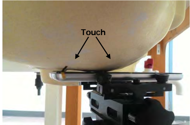
Fig.3 Right Head Section / Cheek-Touch Position
