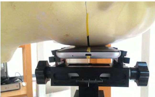
Fig.5 Left Head Section / Cheek-Touch Position
