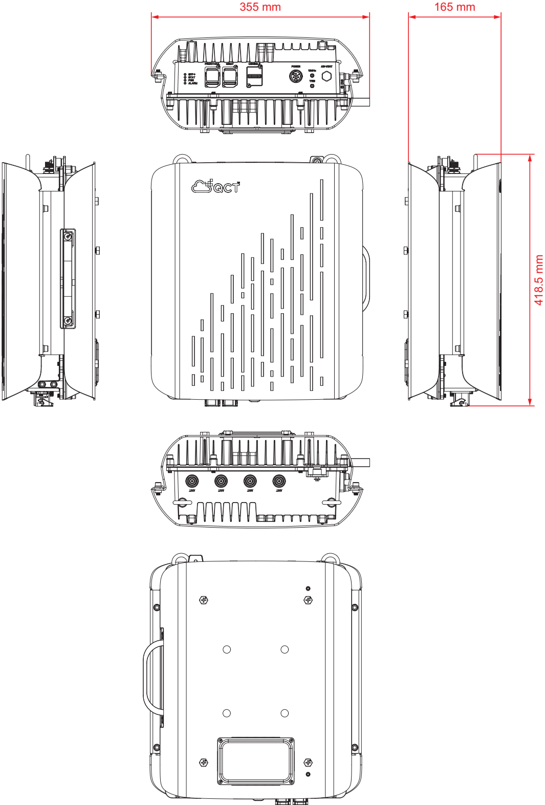
Figure 1-6. System Dimensions
