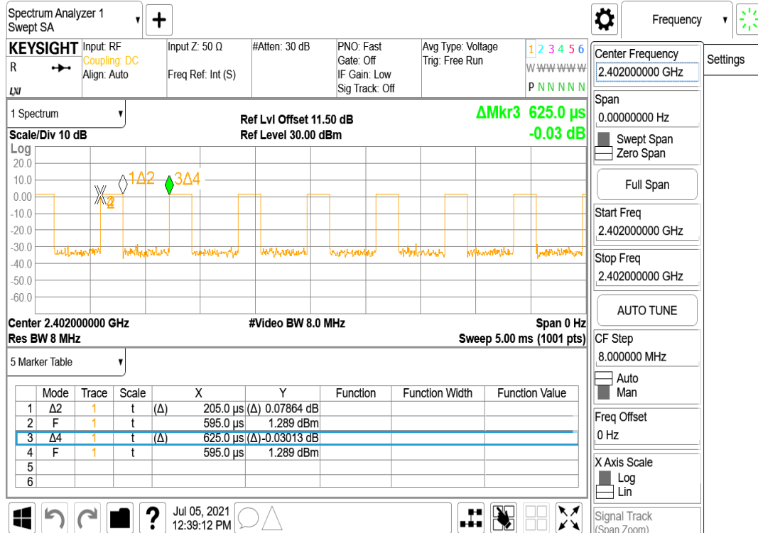
BLE_2M_LowCH00-2402
