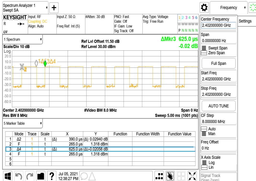
BLE_1M_LowCH00-2402
