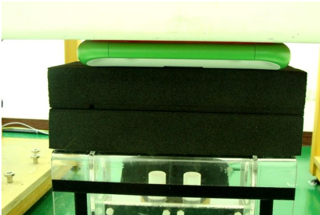
Bottom of Tablet – Antenna Position 0°
