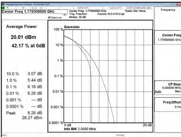
Band66_1.4MHz_16QAM_RB6_0_CH132665
