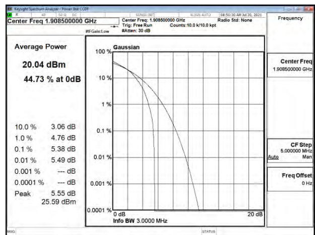
Band2_3MHz_16QAM_RB15_0_CH19185
