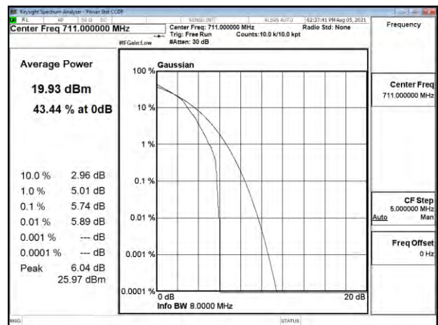
Band17_10MHz_16QAM_RB16_0_CH23800
