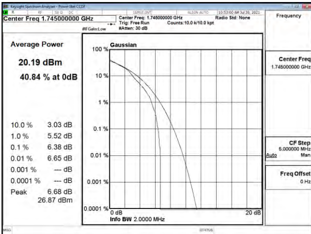
Band66_1.4MHz_16QAM_RB6_0_CH132322
