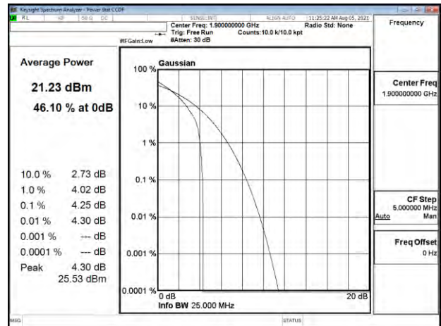
Band2_20MHz_16QAM_RB18_0_CH19100
