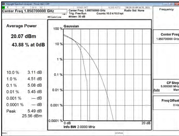
Band2_1.4MHz_16QAM_RB6_0_CH18607
