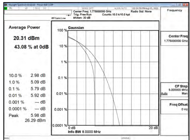
Band66_10MHz_16QAM_RB16_0_CH132622
