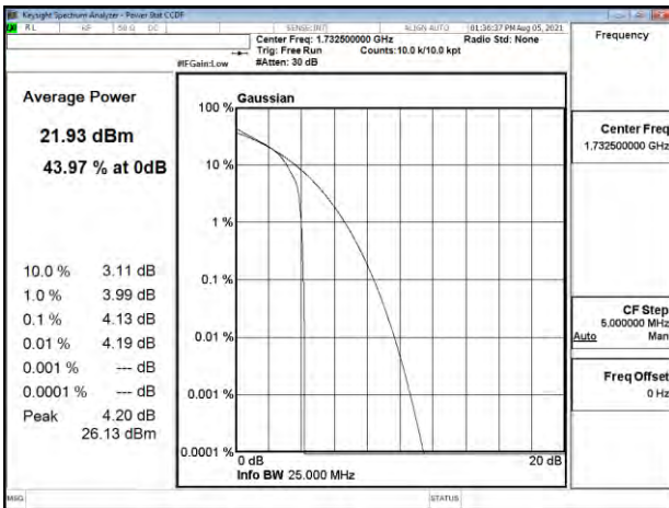
Band4_15MHz_16QAM_RB16_0_CH20175
