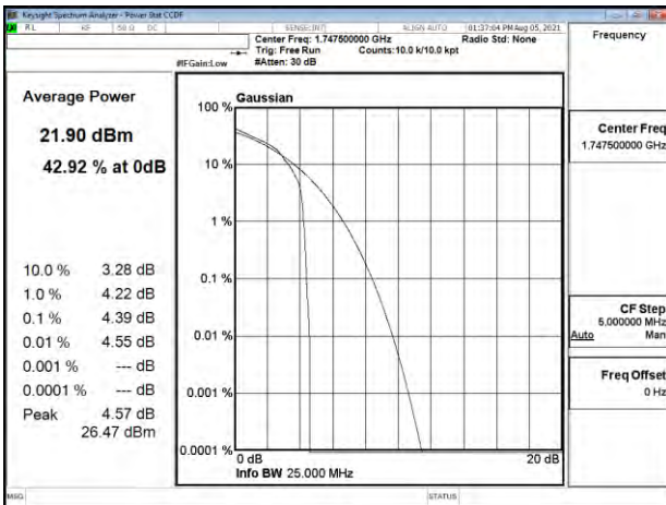
Band4_15MHz_16QAM_RB16_0_CH20325
