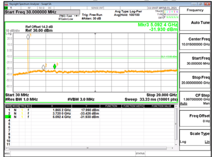
Spurious Emission\Band2_20MHz\QPSK_RB1_0_CH18700
