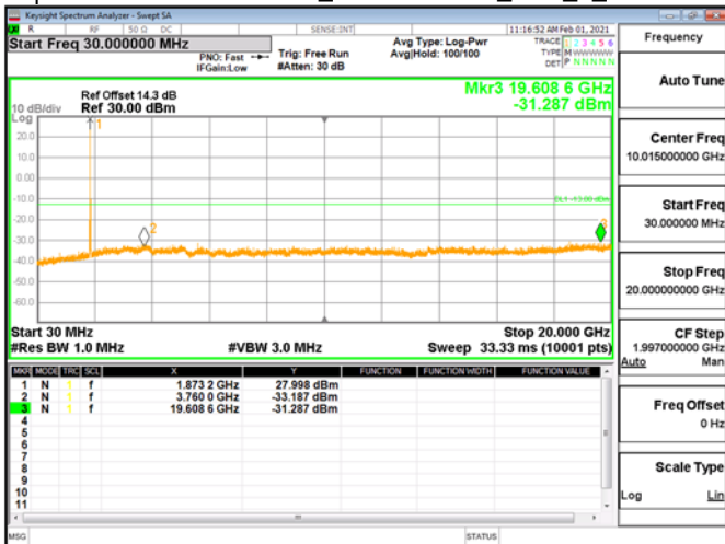
Spurious Emission\Band2_15MHz\QPSK_RB1_0_CH18900
