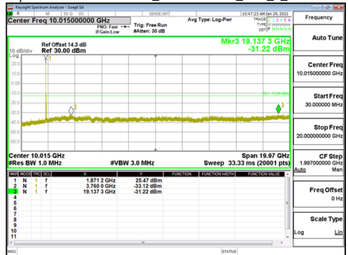
Spurious Emission\Band2_20MHz\QPSK_RB1_0_CH18900
