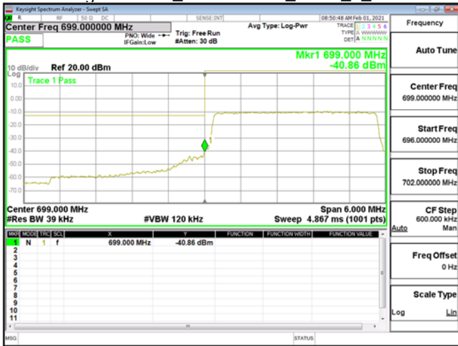
Band Edge\Band12_3MHz\QPSK_RB15_0_CH23025
