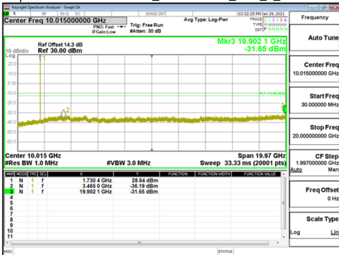
Spurious Emission\Band4_5MHz\QPSK_RB1_0_CH20175
