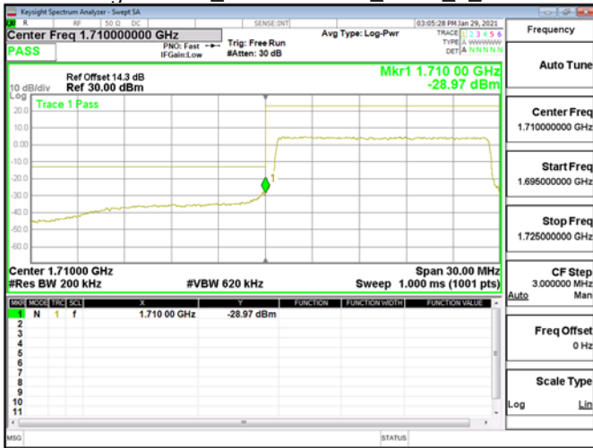
Band Edge\Band4_15MHz\QPSK_RB75_0_CH20025
