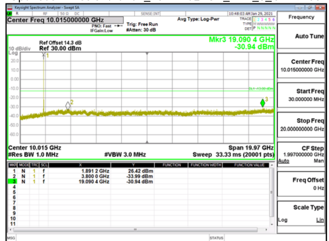
Spurious Emission\Band2_20MHz\QPSK_RB1_0_CH19100
