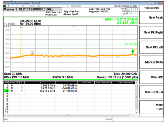
Spurious Emission\Band4_3MHz\QPSK_RB1_0_CH19965
