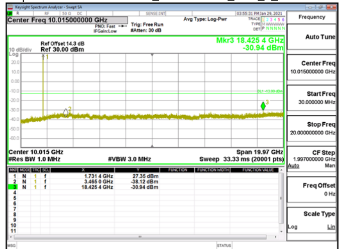
Spurious Emission\Band4_3MHz\QPSK_RB1_0_CH20175
