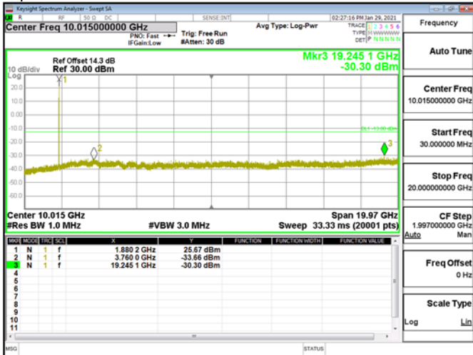
Spurious Emission\Band2_1.4MHz\QPSK_RB1_0_CH18900
