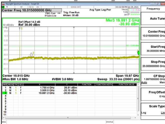
Spurious Emission\Band4_5MHz\QPSK_RB1_0_CH20375
