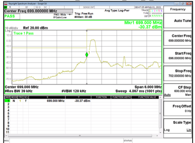
Band Edge\Band12_3MHz\QPSK_RB1_0_CH23025
