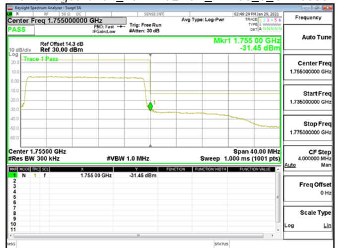
Band Edge\Band4_20MHz\QPSK_RB100_0_CH20300
