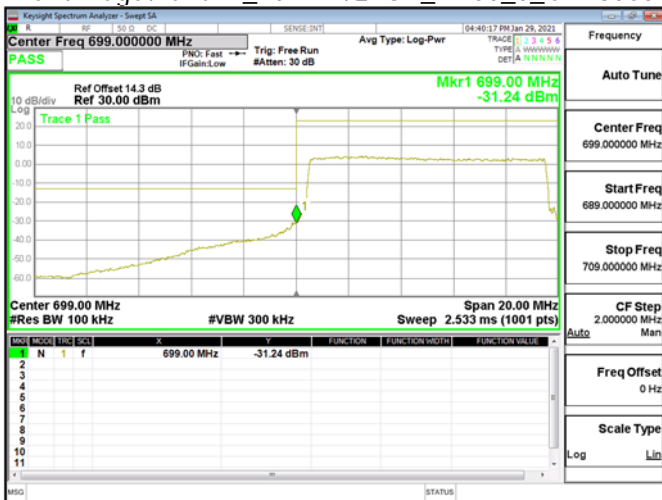
Band Edge\Band12_10MHz\QPSK_RB50_0_CH23060
