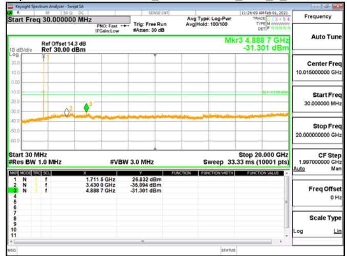
Spurious Emission\Band4_10MHz\QPSK_RB1_0_CH20000
