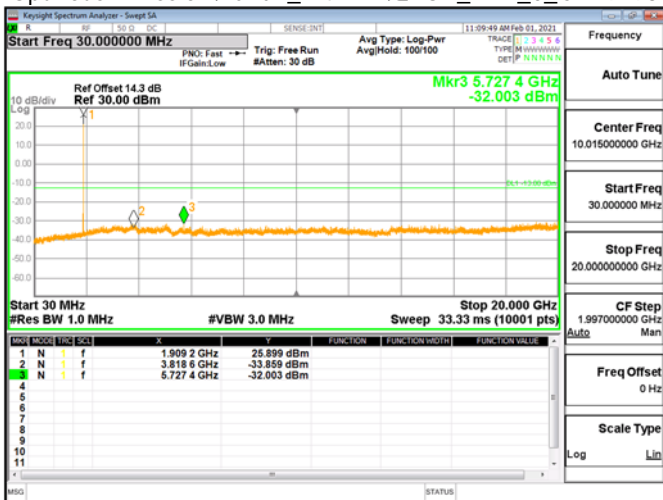
Spurious Emission\Band2_1.4MHz\QPSK_RB1_0_CH19193
