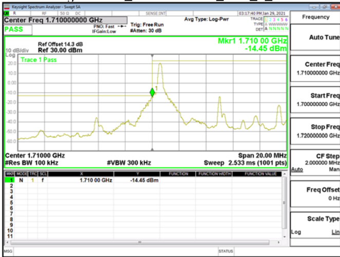
Band Edge\Band4_10MHz\QPSK_RB1_0_CH20000
