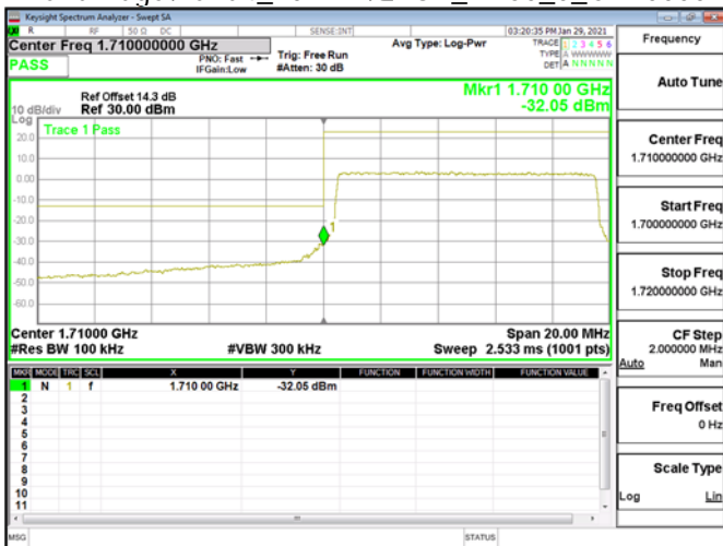
Band Edge\Band4_10MHz\QPSK_RB50_0_CH20000
