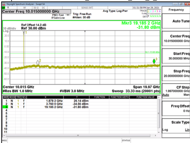
Spurious Emission\Band2_5MHz\QPSK_RB1_0_CH18900
