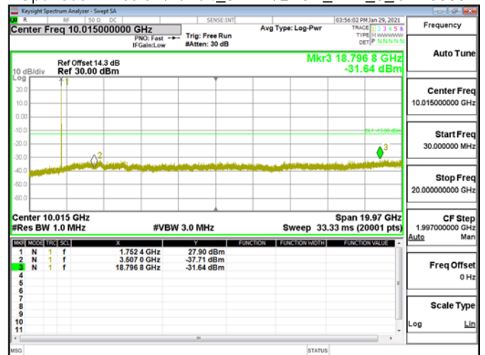
Spurious Emission\Band4_3MHz\QPSK_RB1_0_CH20385
