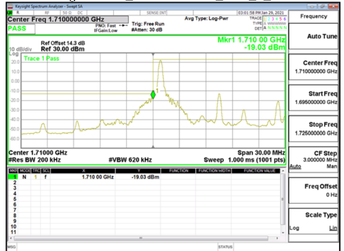
Band Edge\Band4_15MHz\QPSK_RB1_0_CH20025
