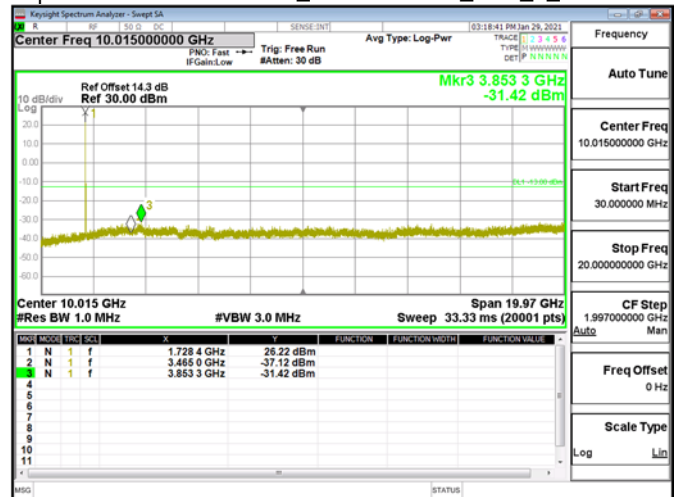
Spurious Emission\Band4_10MHz\QPSK_RB1_0_CH20175
