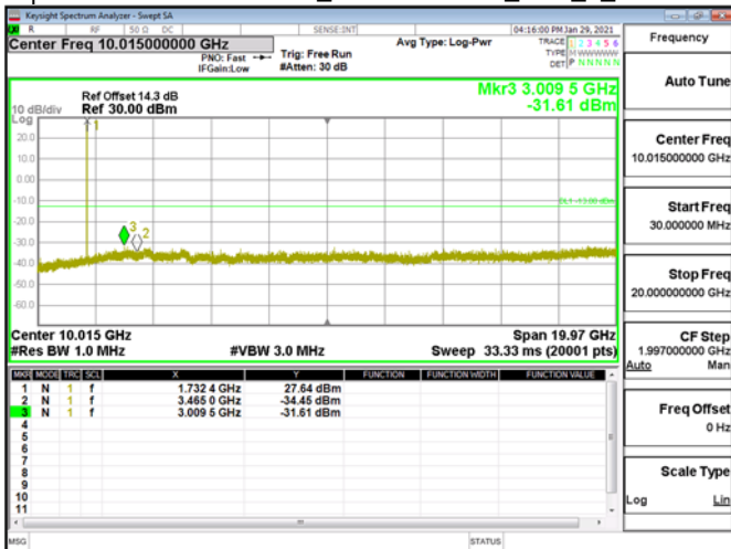
Spurious Emission\Band4_1.4MHz\QPSK_RB1_0_CH20175
