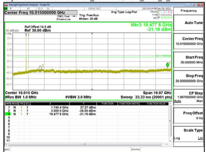
Spurious Emission\Band4_10MHz\QPSK_RB1_0_CH20350
