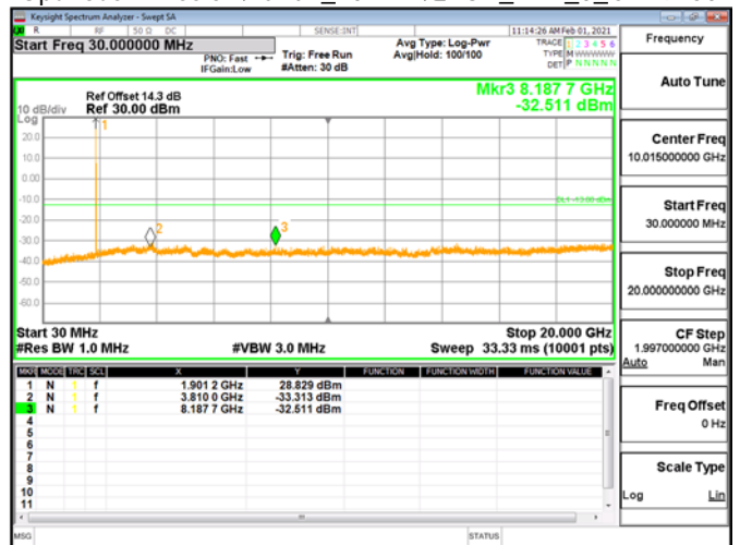
Spurious Emission\Band2_10MHz\QPSK_RB1_0_CH19150
