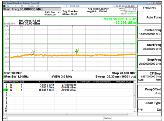
Spurious Emission\Band2_3MHz\QPSK_RB1_0_CH18615
