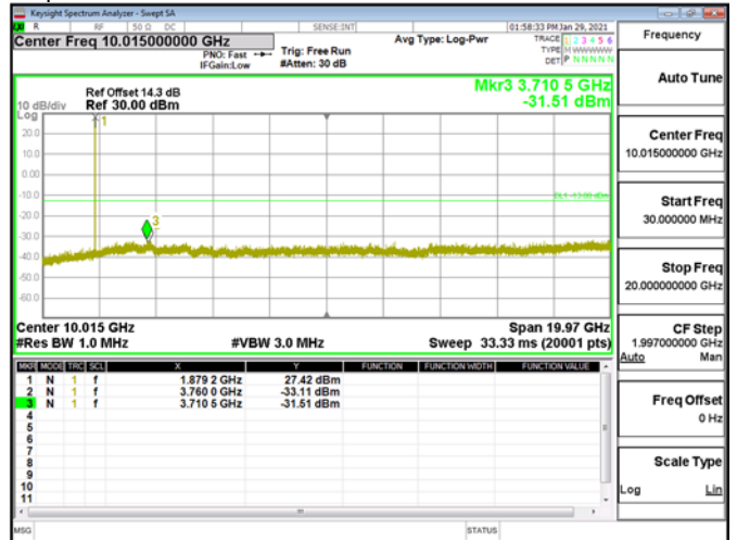
Spurious Emission\Band2_3MHz\QPSK_RB1_0_CH18900
