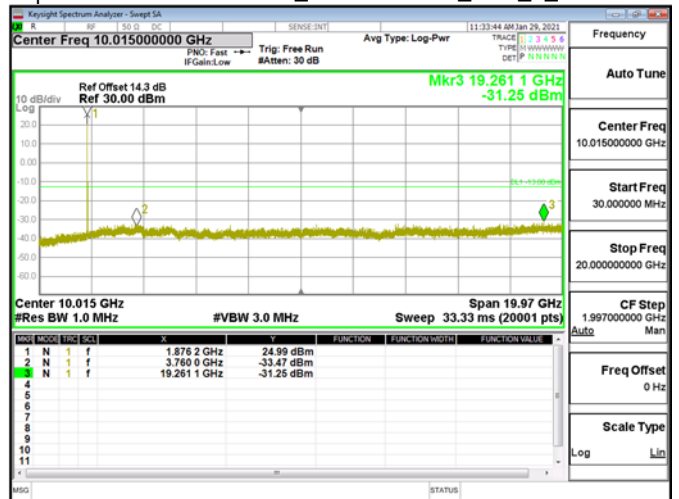
Spurious Emission\Band2_10MHz\QPSK_RB1_0_CH18900
