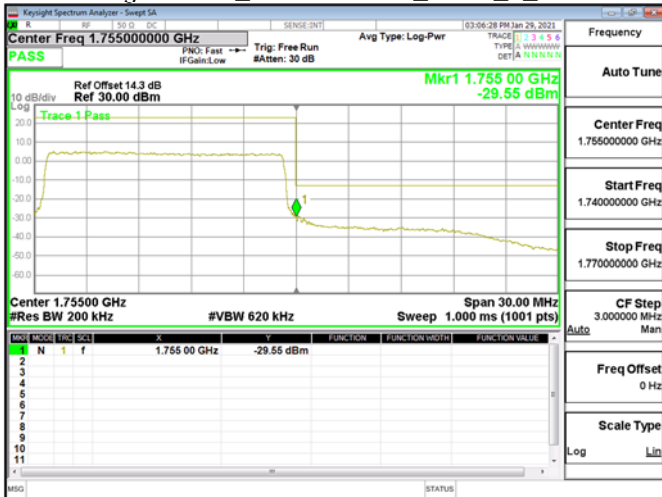
Band Edge\Band4_15MHz\QPSK_RB75_0_CH20325
