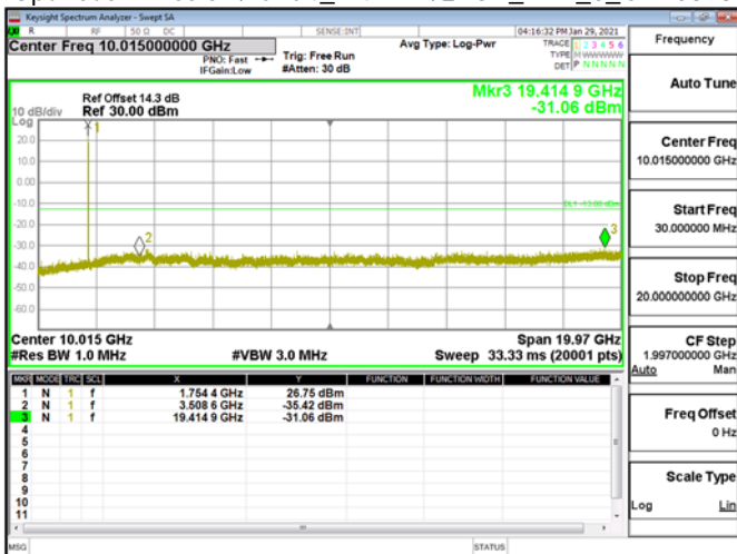
Spurious Emission\Band4_1.4MHz\QPSK_RB1_0_CH20393
