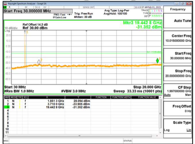
Spurious Emission\Band2_10MHz\QPSK_RB1_0_CH18650
