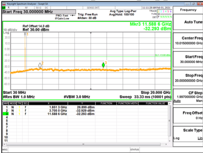
Spurious Emission\Band2_5MHz\QPSK_RB1_0_CH18625
