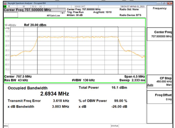
OBWBand12_3MHz\16QAM_RB15_0_CH23095
