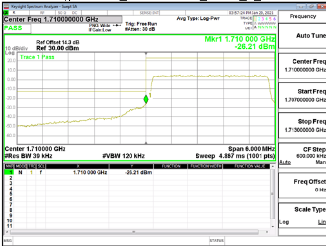
Band Edge\Band4_3MHz\QPSK_RB15_0_CH19965
