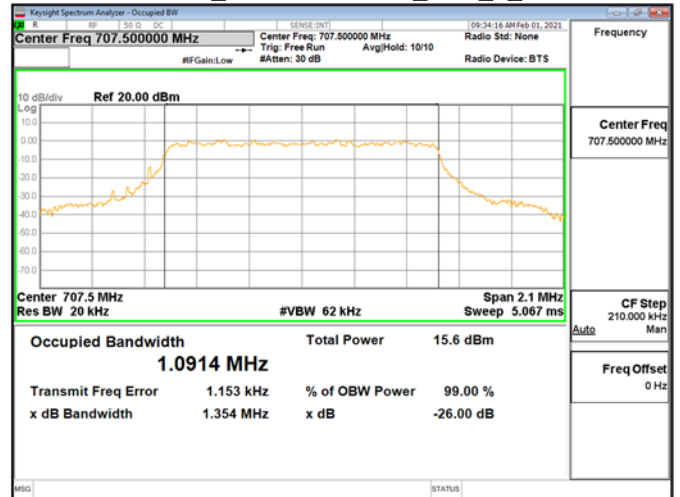
OBWBand12_1.4MHz\16QAM_RB6_0_CH23095
