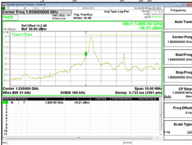
Band Edge\Band2_5MHz\QPSK_RB1_0_CH18625
