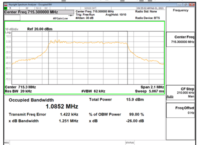
OBWBand12_1.4MHz\16QAM_RB6_0_CH23173
