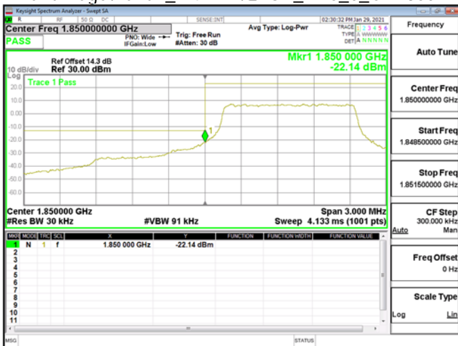
Band Edge\Band2_1.4MHz\QPSK_RB6_0_CH18607
