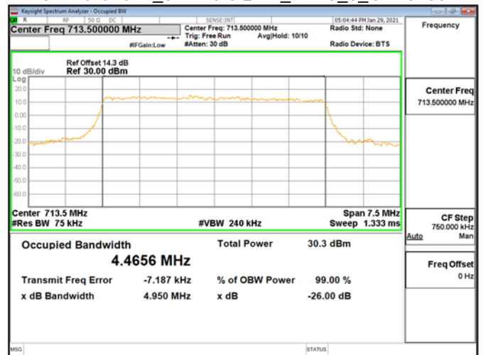
OBWBand12_5MHz\16QAM_RB25_0_CH23155
