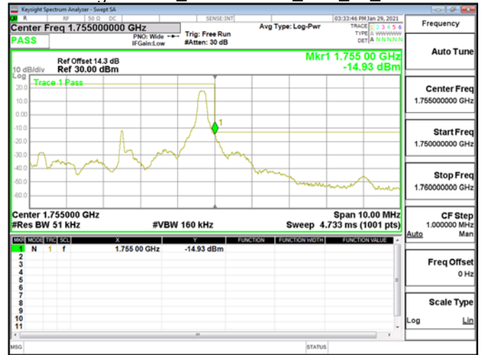
Band Edge\Band4_5MHz\QPSK_RB1_24_CH20375
