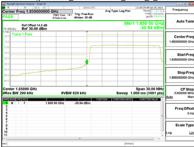
Band Edge\Band2_15MHz\QPSK_RB75_0_CH18675
