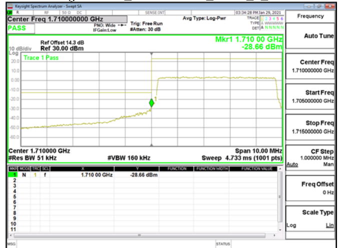
Band Edge\Band4_5MHz\QPSK_RB25_0_CH19975
