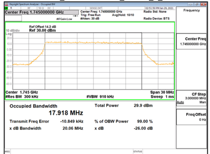
OBWBand4_20MHz\16QAM_RB100_0_CH20300
