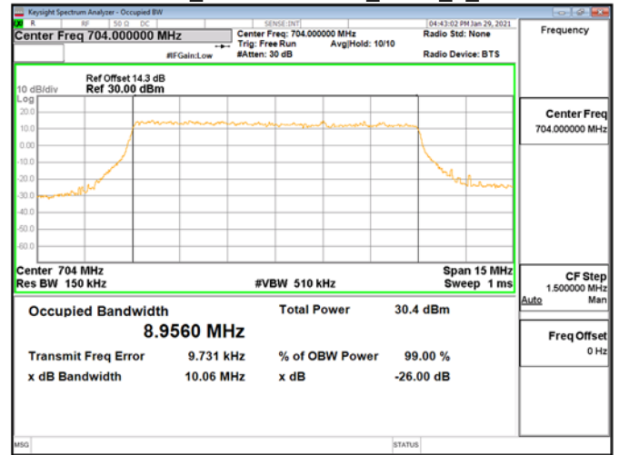
OBWBand12_10MHz\16QAM_RB50_0_CH23060
