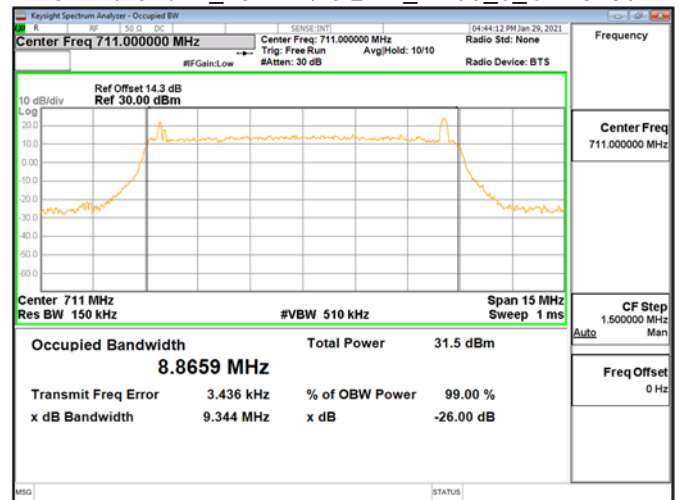
OBWBand12_10MHz\16QAM_RB50_0_CH23130
