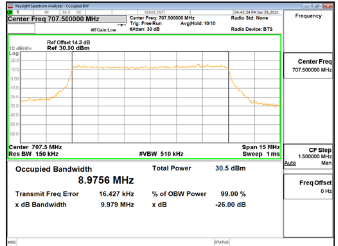
OBWBand12_10MHz\16QAM_RB50_0_CH23095
