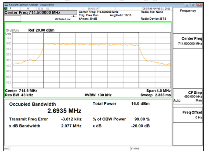
OBWBand12_3MHz\16QAM_RB15_0_CH23165
