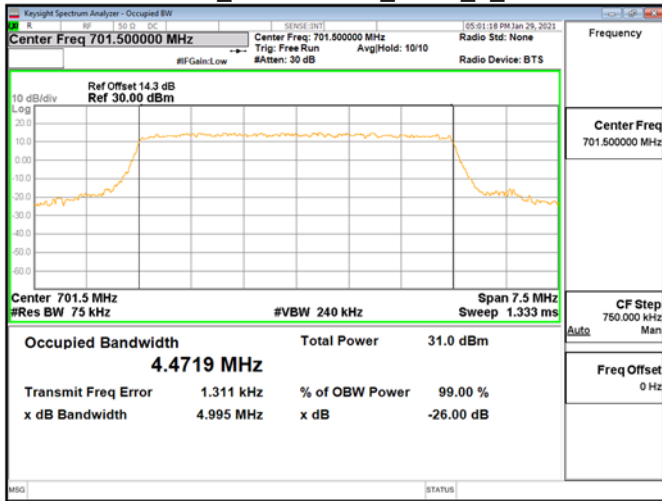
OBWBand12_5MHzQPSK_RB25_0_CH23035
