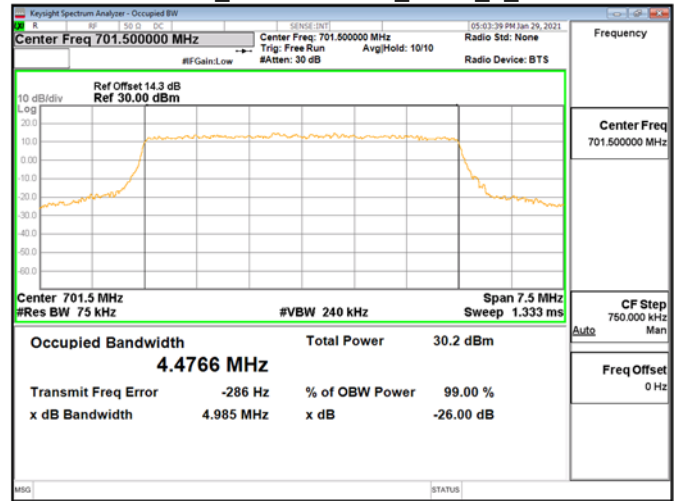
OBWBand12_5MHz\16QAM_RB25_0_CH23035
