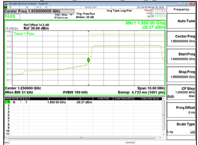
Band Edge\Band2_5MHz\QPSK_RB25_0_CH18625
