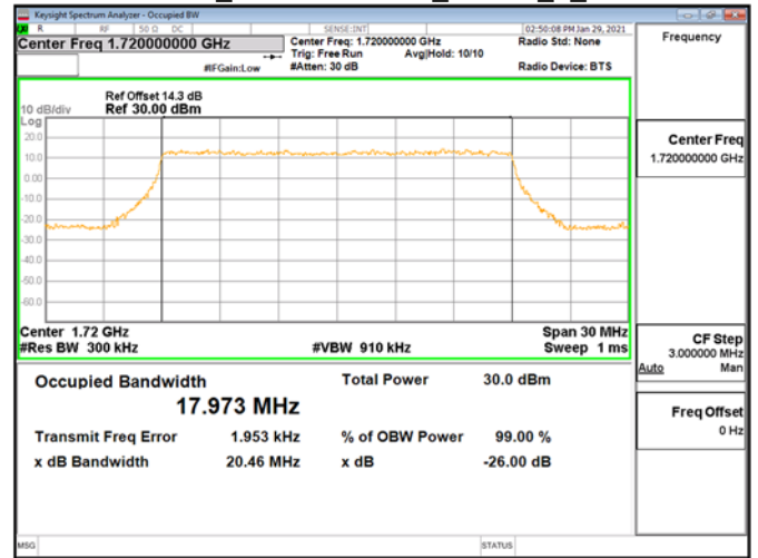
OBWBand4_20MHz\16QAM_RB100_0_CH20050
