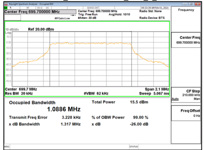
OBWBand12_1.4MHz\16QAM_RB6_0_CH23017
