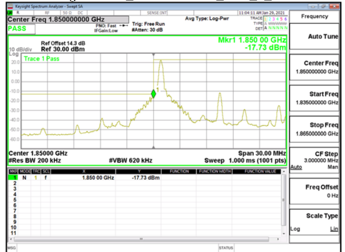
Band Edge\Band2_15MHz\QPSK_RB1_0_CH18675
