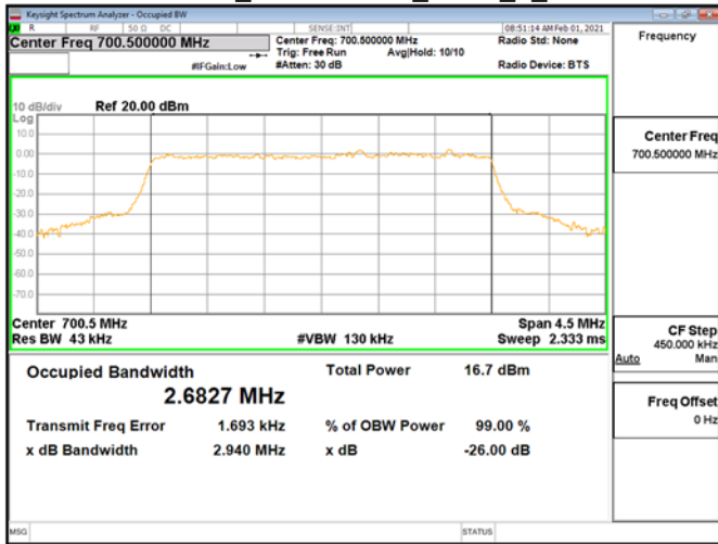
OBWBand12_3MHzQPSK_RB15_0_CH23025
