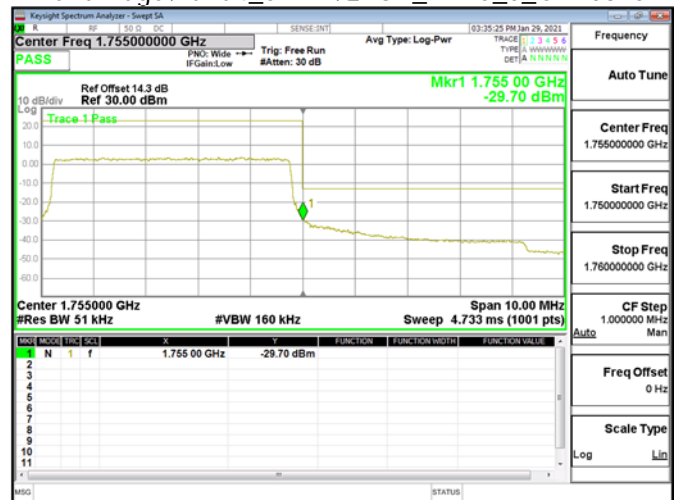
Band Edge\Band4_5MHz\QPSK_RB25_0_CH20375
