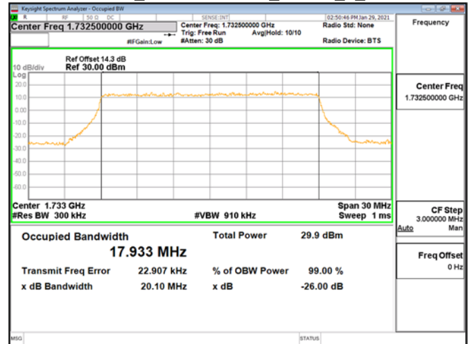
OBWBand4_20MHz\16QAM_RB100_0_CH20175
