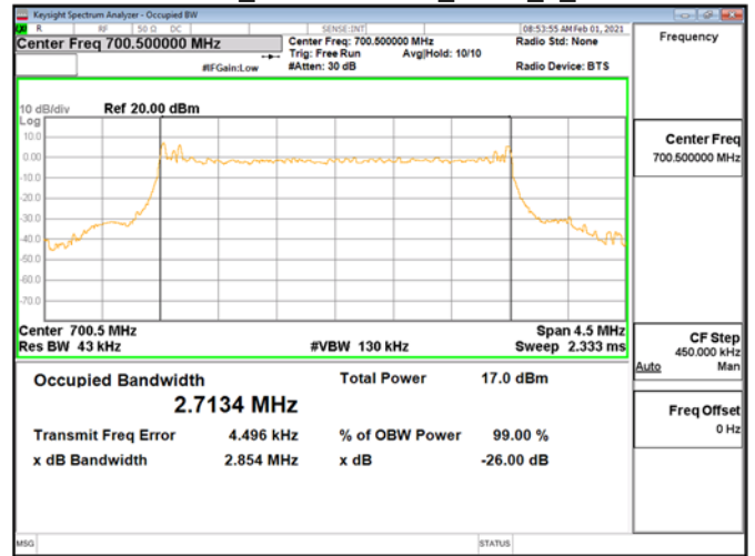
OBWBand12_3MHz\16QAM_RB15_0_CH23025
