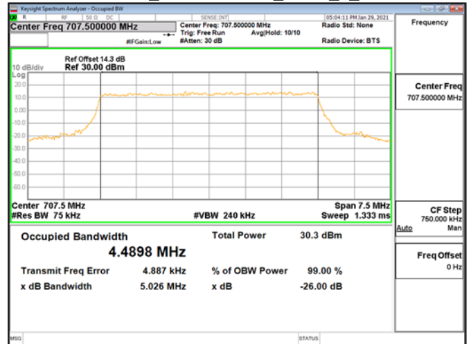
OBWBand12_5MHz\16QAM_RB25_0_CH23095
