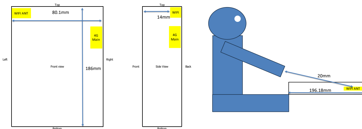
Photograph 17. Antenna position of EUT
