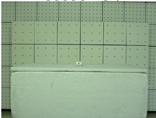
Part_22_24_27_4G_Radiated_Setup
