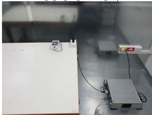
Part_15_225_NFC_Conduction_Setup
