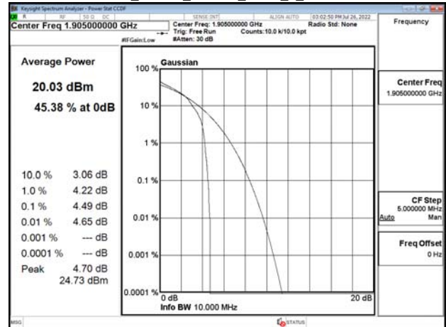
Band2_10MHz_16QAM_RB27_0_CH19150
