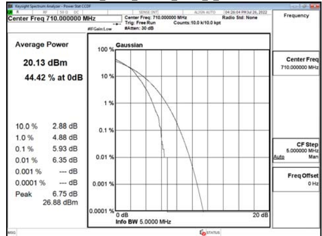
Band17_5MHz_16QAM_RB25_0_CH23790
