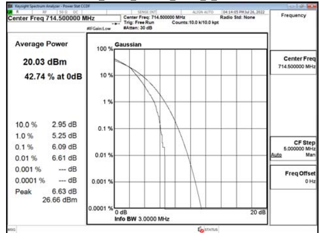
Band12_3MHz_16QAM_RB15_0_CH23165
