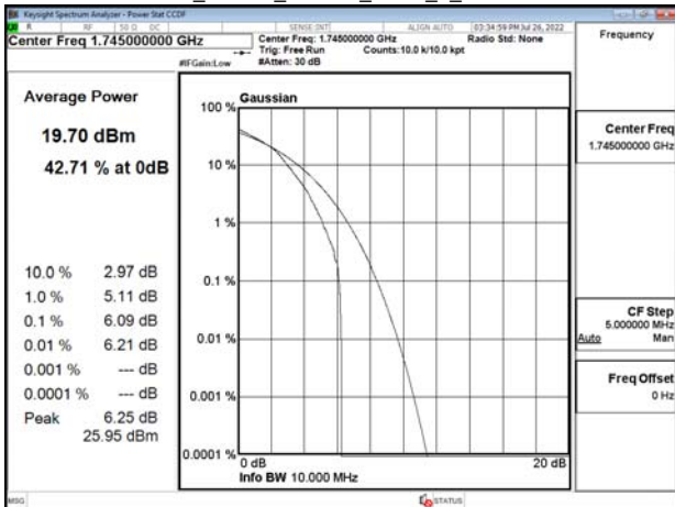
Band66_10MHz_16QAM_RB27_0_CH132322
