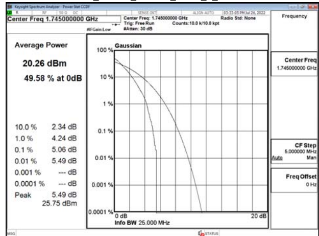
Band66_15MHz_16QAM_RB75_0_CH132322
