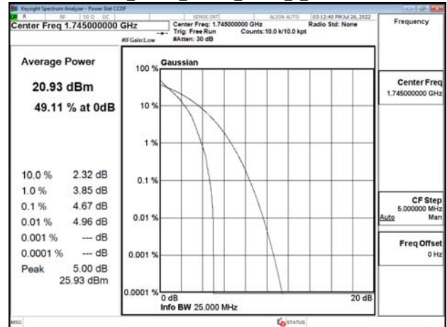
Band4_20MHz_16QAM_RB100_0_CH20300
