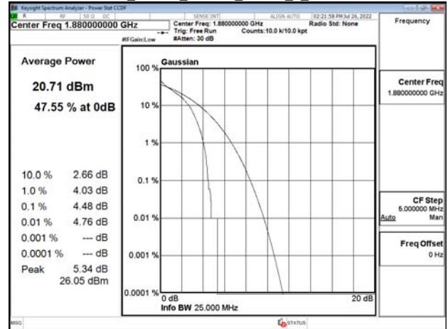
Band2_20MHz_16QAM_RB100_0_CH19100
