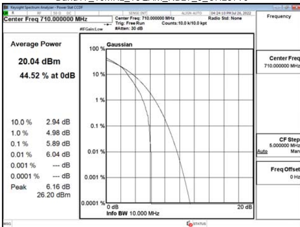
Band17_10MHz_16QAM_RB27_0_CH23790
