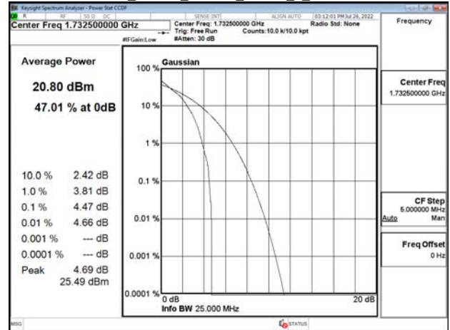
Band4_20MHz_16QAM_RB100_0_CH20300
