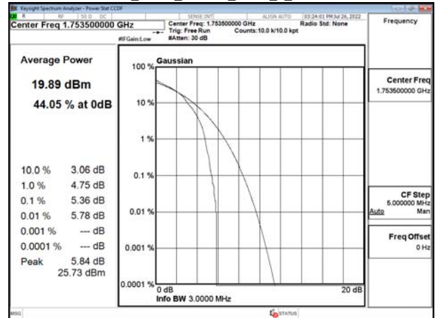
Band4_3MHz_16QAM_RB15_0_CH20385
