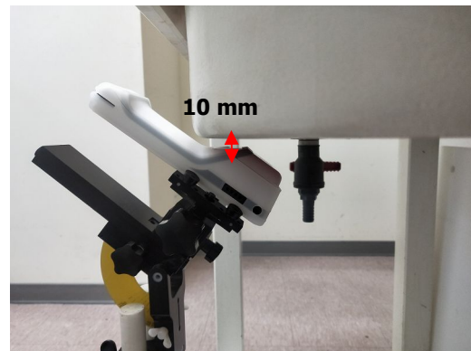
Photograph 4. EUT Back side to flat phantom
