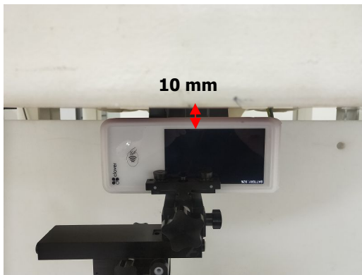
Photograph 9. EUT Bottom side to flat phantom
