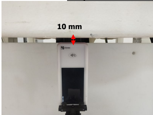
Photograph 7. EUT Top side to flat phantom
