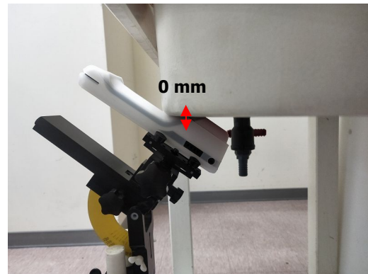
Photograph 20. EUT Back (curve) side to flat phantom
