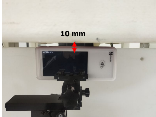
Photograph 13. EUT Left side to flat phantom
