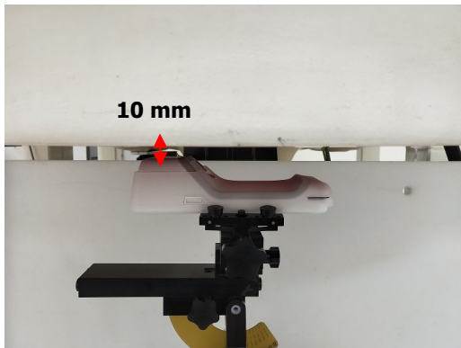
Photograph 1. EUT Front side to flat phantom
