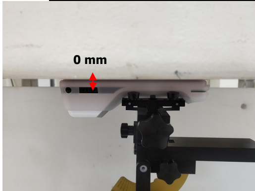
Photograph 15. EUT Front side to flat phantom
