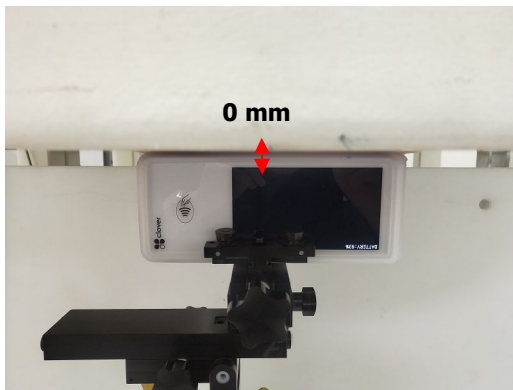
Photograph 23. EUT Bottom side to flat phantom
