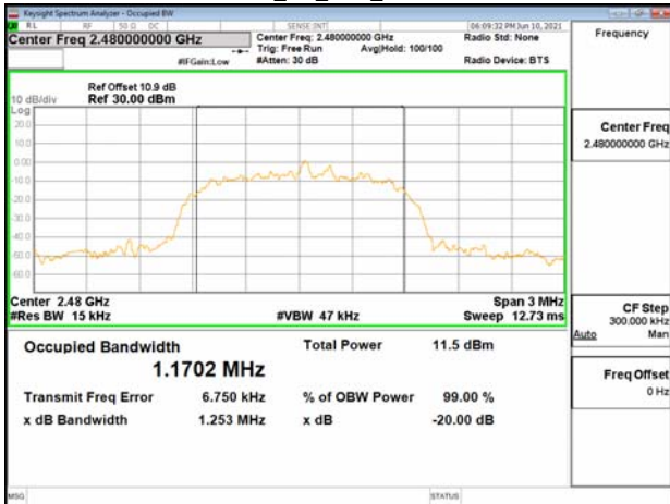
8DPSK_3M_DH5_2480MHz
