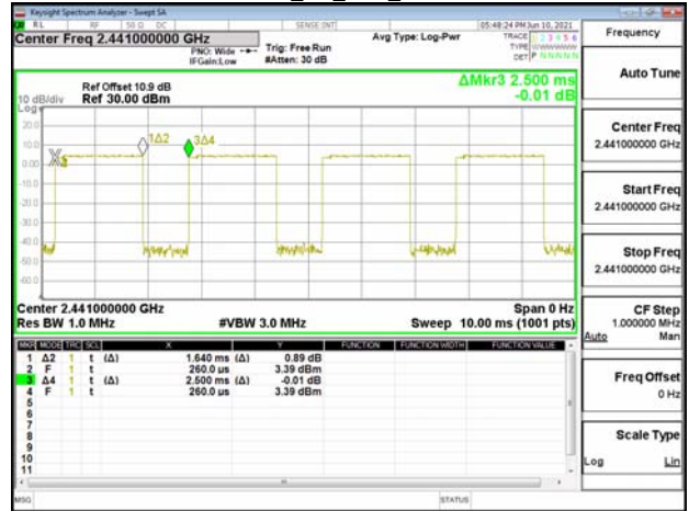
4DQPSK_2M_DH5_2441MHz
