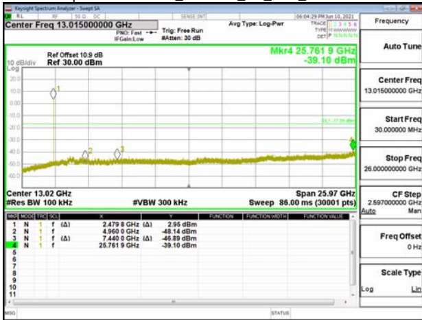
Spurious Emission_4DQPSK_2M_DH5_2480MHz
