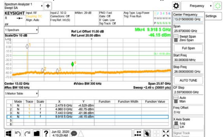
BLE 2M\Spurious Emission_BLE_2M_HighCH39-2480
