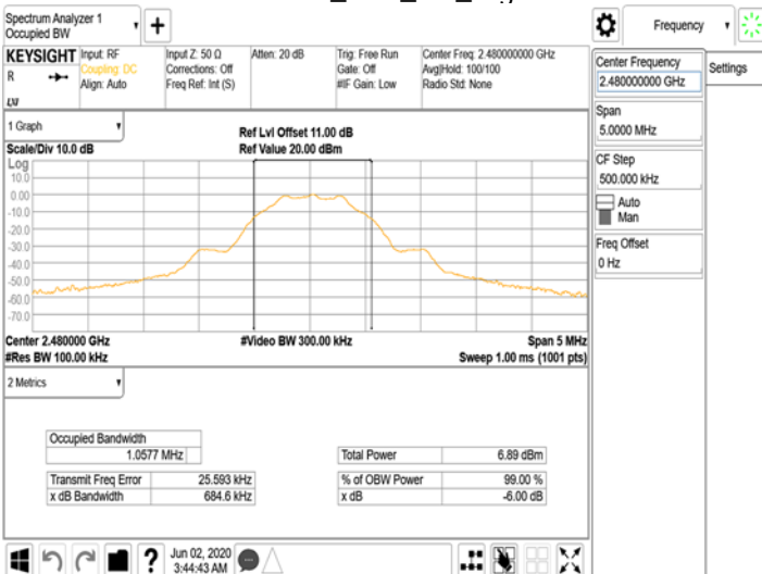
BLE 1M0BW 6dB_BLE_1M_HighCH39-2480
