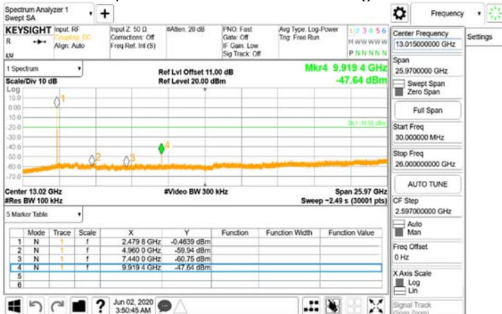
BLE 1M\Spurious Emission_BLE_1M_HighCH39-2480
