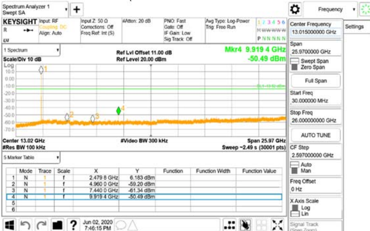
FCC_15_247_BTSpurious Emission_GFSK_1M_DH5_2480MHz
