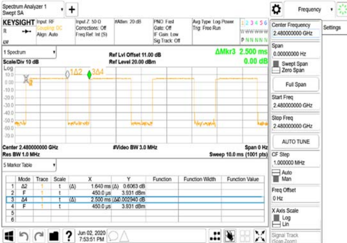
FCC_15_247_BTWdwell Time_π/4DQPSK_2M_2480MHz
