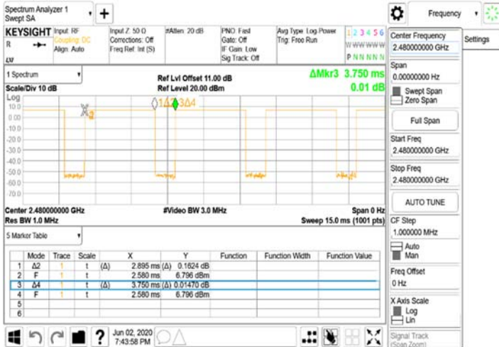
FCC_15_247_BT\Dwell Time_GFSK_1M_DH5_2480MHz
