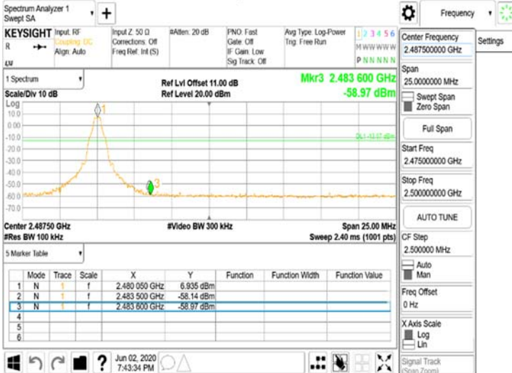
FCC_15_247_BTBand Edge_GFSK_1M_DH5_2480MHz
