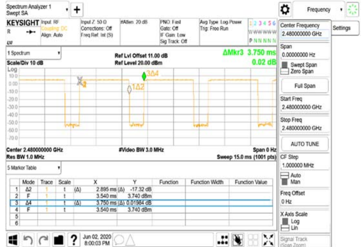
FCC_15_247_BTWdwell Time_π/4DQPSK_2M_2480MHz
