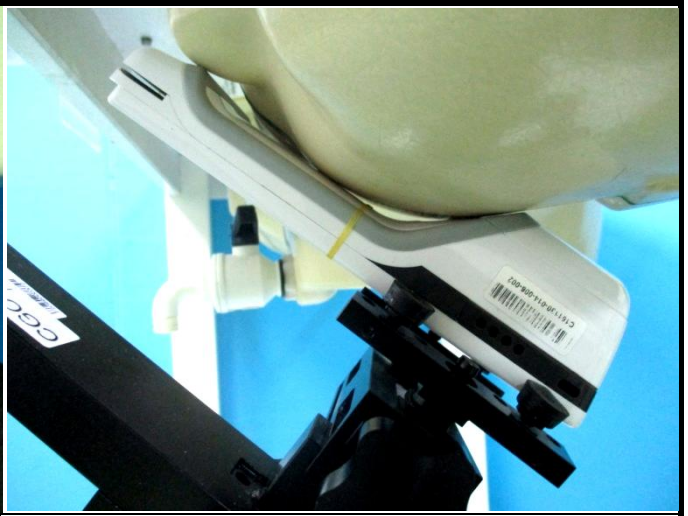
Left Face of EUT with 0 cm Gap
