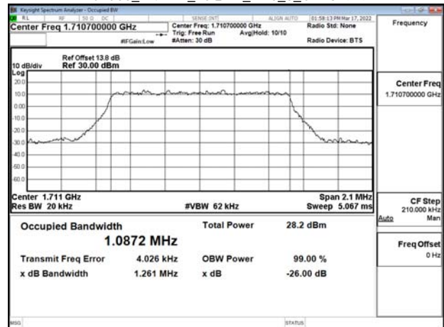
Band66_1.4MHz_16QAM_RB6_0_CH131979
