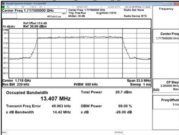
Band66_15MHz_QPSK_RB75_0_CH132047
