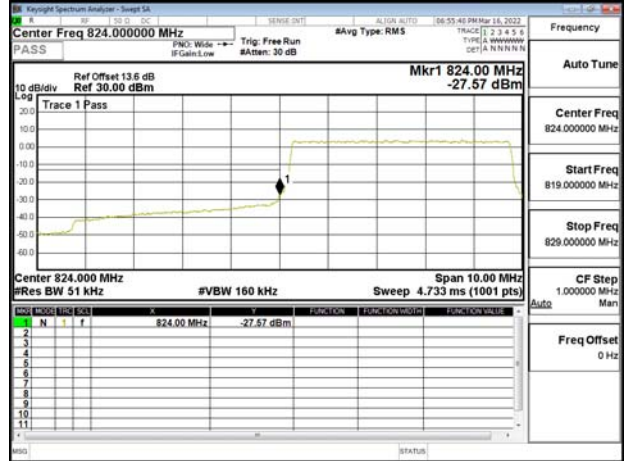
Band Edge_Band5_5MHz_OPSK_RB25_0_CH20625
