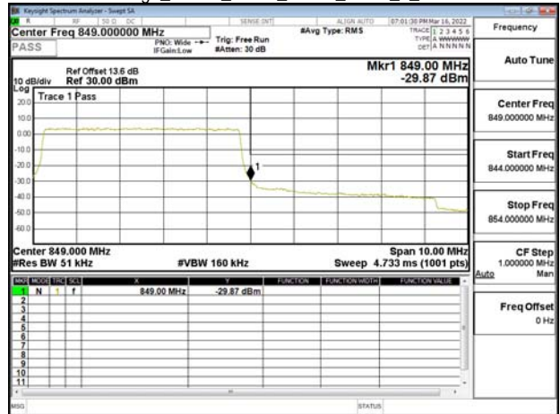
Band Edge_Band5_5MHz_OPSK_RB25_0_CH20625
