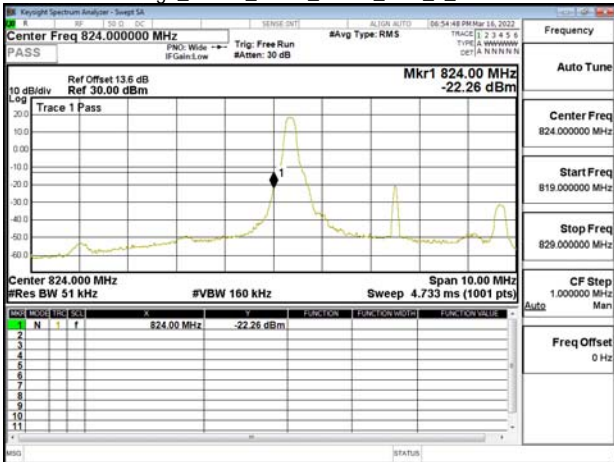
Band Edge_Band5_5MHz_OPSK_RB1_0_CH20425
