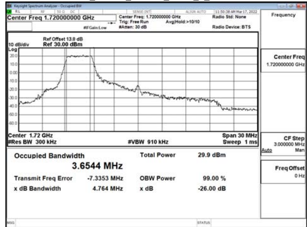
Band66_20MHz_16QAM_RB18_0_CH132072
