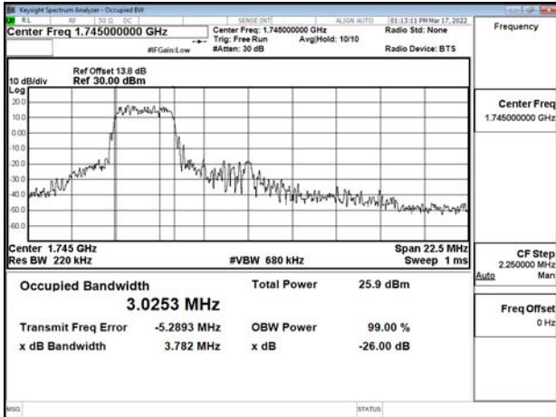
Band66_15MHz_16QAM_RB16_0_CH132597
