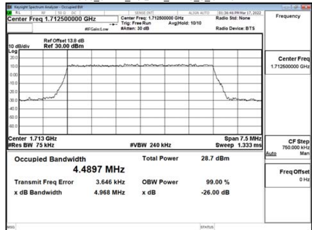
Band66_5MHz_16QAM_RB25_0_CH131997
