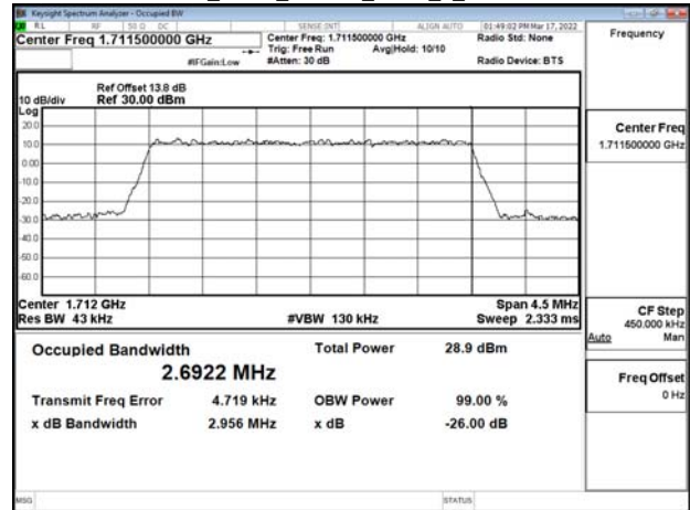
Band66_3MHz_16QAM_RB15_0_CH131987
