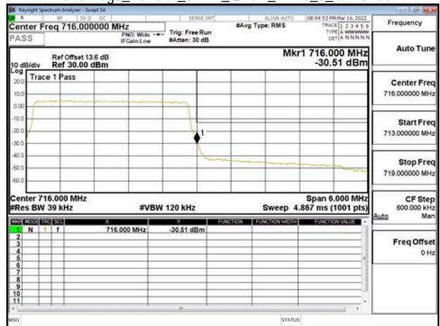
Band Edge_Band12_3MHz_QPSK_RB15_0_CH23165
