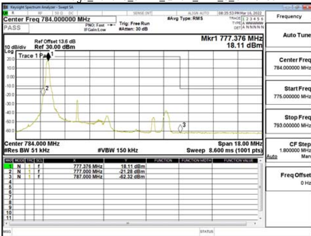
Band Edge_Band13_5MHz_QPSK_RB1_0_CH23205
