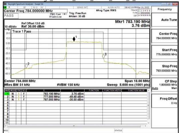
Band Edge_Band13_5MHz_QPSK_RB25_0_CH23255
