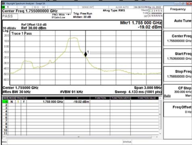
Band Edge_Band4_1.4MHz_QPSK_RB6_0_CH19957
