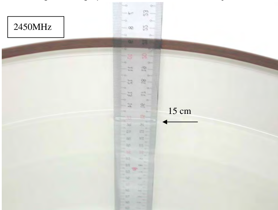
Fig.2 Photograph of the Tissue Simulant liquid depth 15cm
