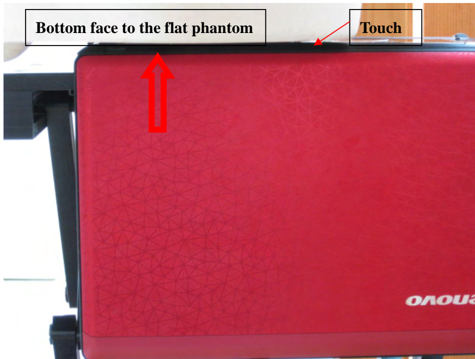
Fig.3 Bottom side of the Netbook is paralleled with flat phantom, open the panel with 90 degrees, bottom side is contact with flat phantom.
