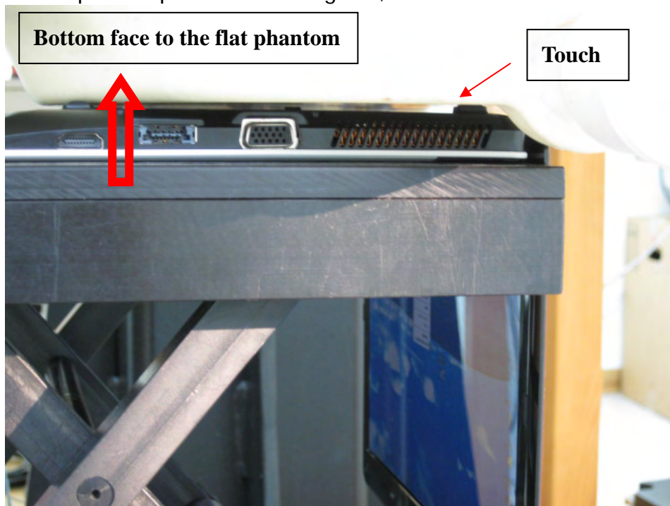
Fig.4 Bottom side of the Netbook is paralleled with flat phantom, open the panel with 90 degrees, bottom side is contact with flat phantom.
