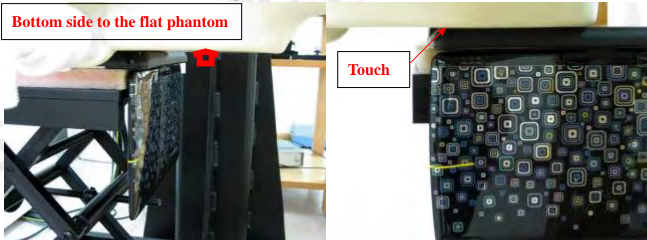
Fig.4 Bottom side of the Notebook is paralleled with flat phantom, open the panel with 90 degrees, bottom side is contact with flat phantom.
