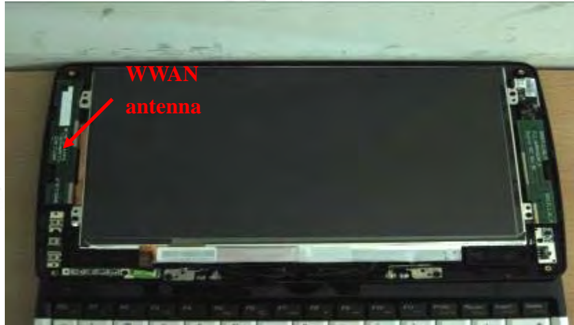
Fig.3 Antenna position of EUT
