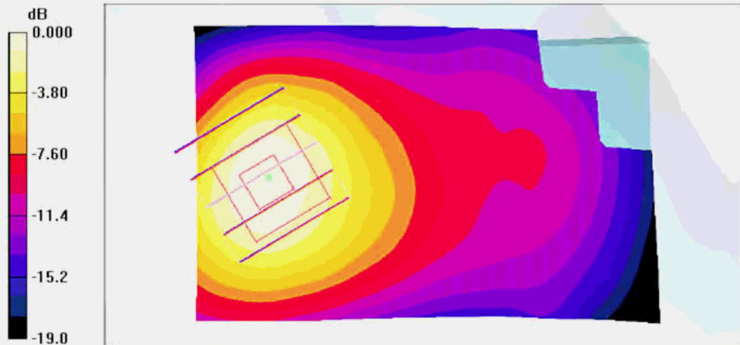
0 dB = 0.634mW/g
