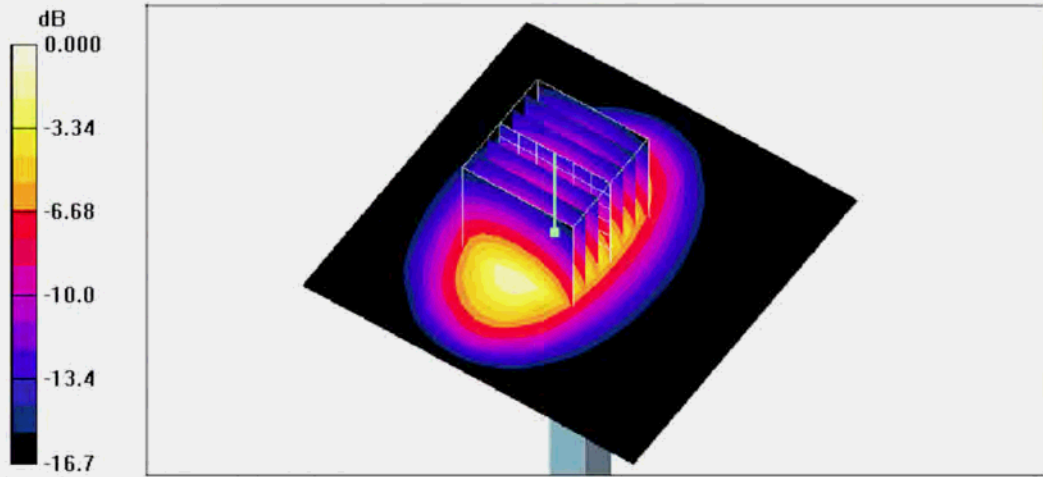
0 dB = 4.42mW/g
