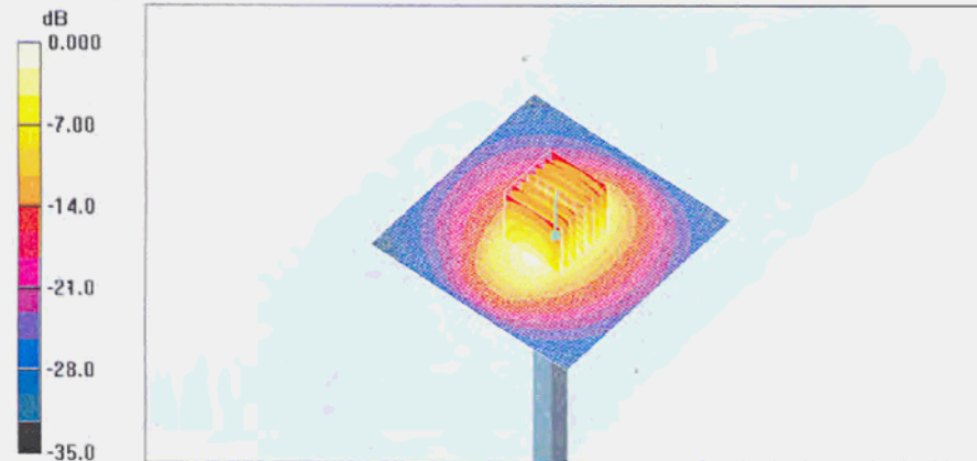
0 dB = 11.6mW/g
