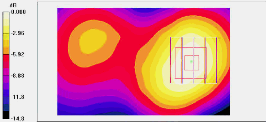
0 dB = 0.862mW/g
