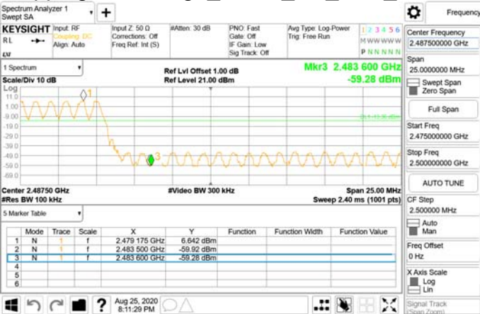
Hopping Band Edge_GFSK_1M_DH5_2480MHz
