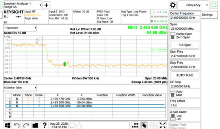
Hopping Band Edge_8DPSK_3M_DH5_2480MHz
