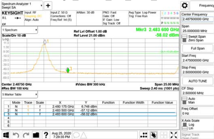
Band Edge_GFSK_1M_DH5_2480MHz
