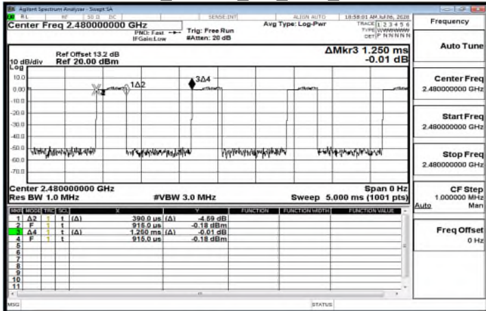
Dwell Time_8DPSK_3M_DH1_2480MHz
