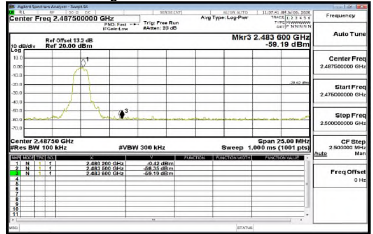
Band Edge_8DPSK_3M_DH5_2480MHz
