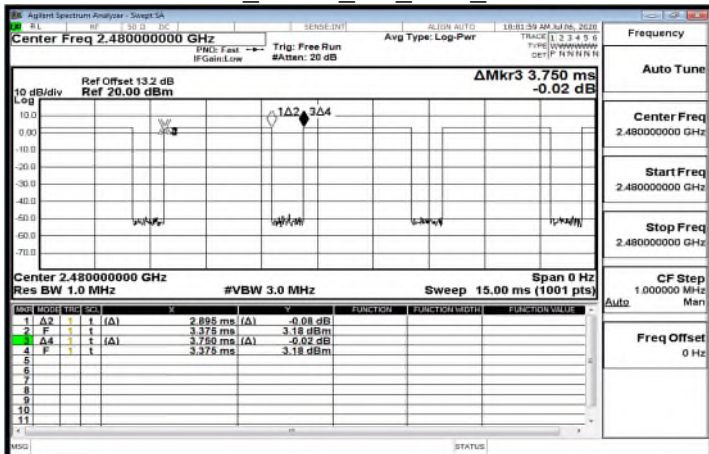
Dwell Time_GFSK_1M_DH5_2480MHz
