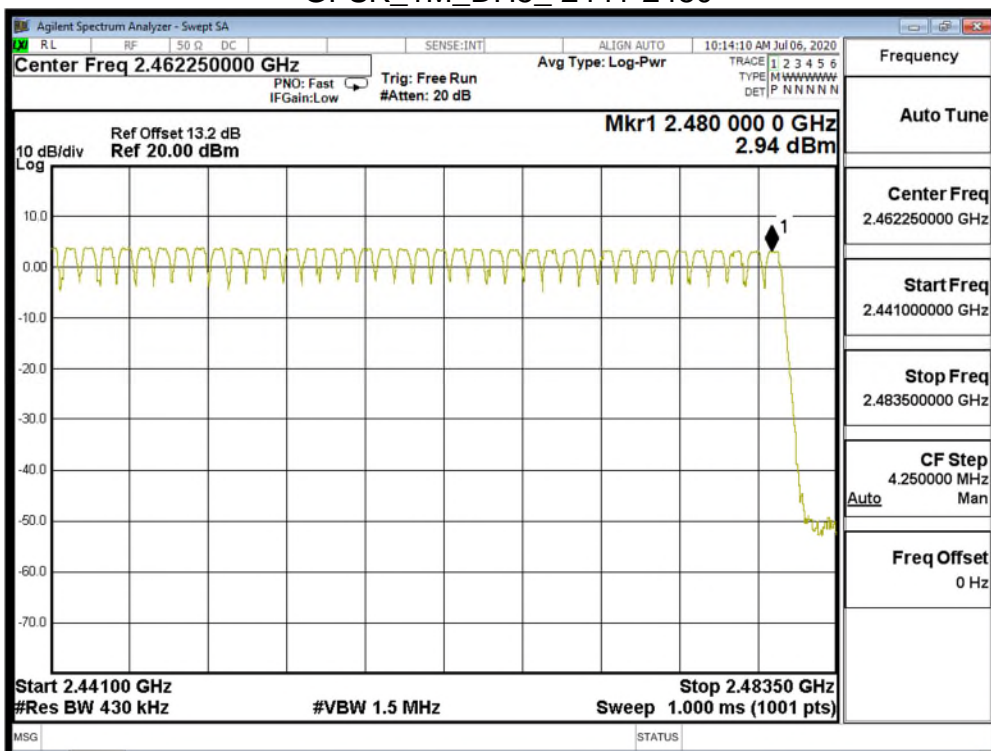
GFSK_1M_DH5_2441-2480
