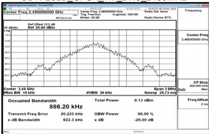
OBW 20dB_GFSK_1M_DH5_2480MHz
