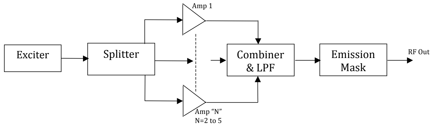
Transmitter Block Diagram
