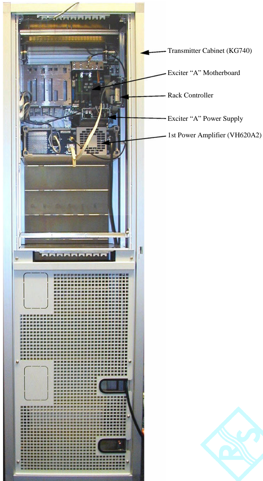
Rear View of Typical SV7000 Full Cabinet Transmitter (with top half of two-piece rear cover removed)
