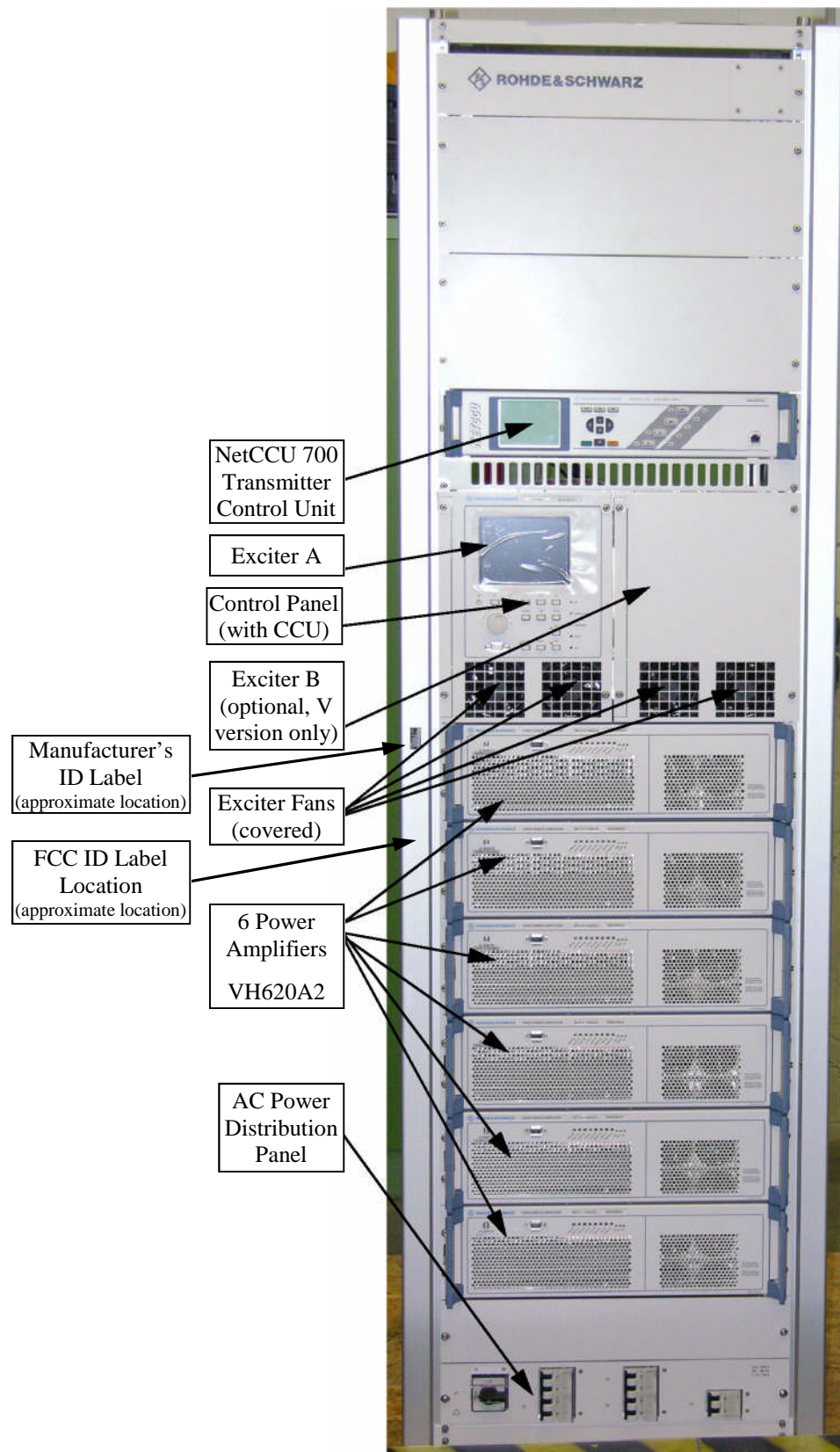
Front View of SV7600 Transmitter
