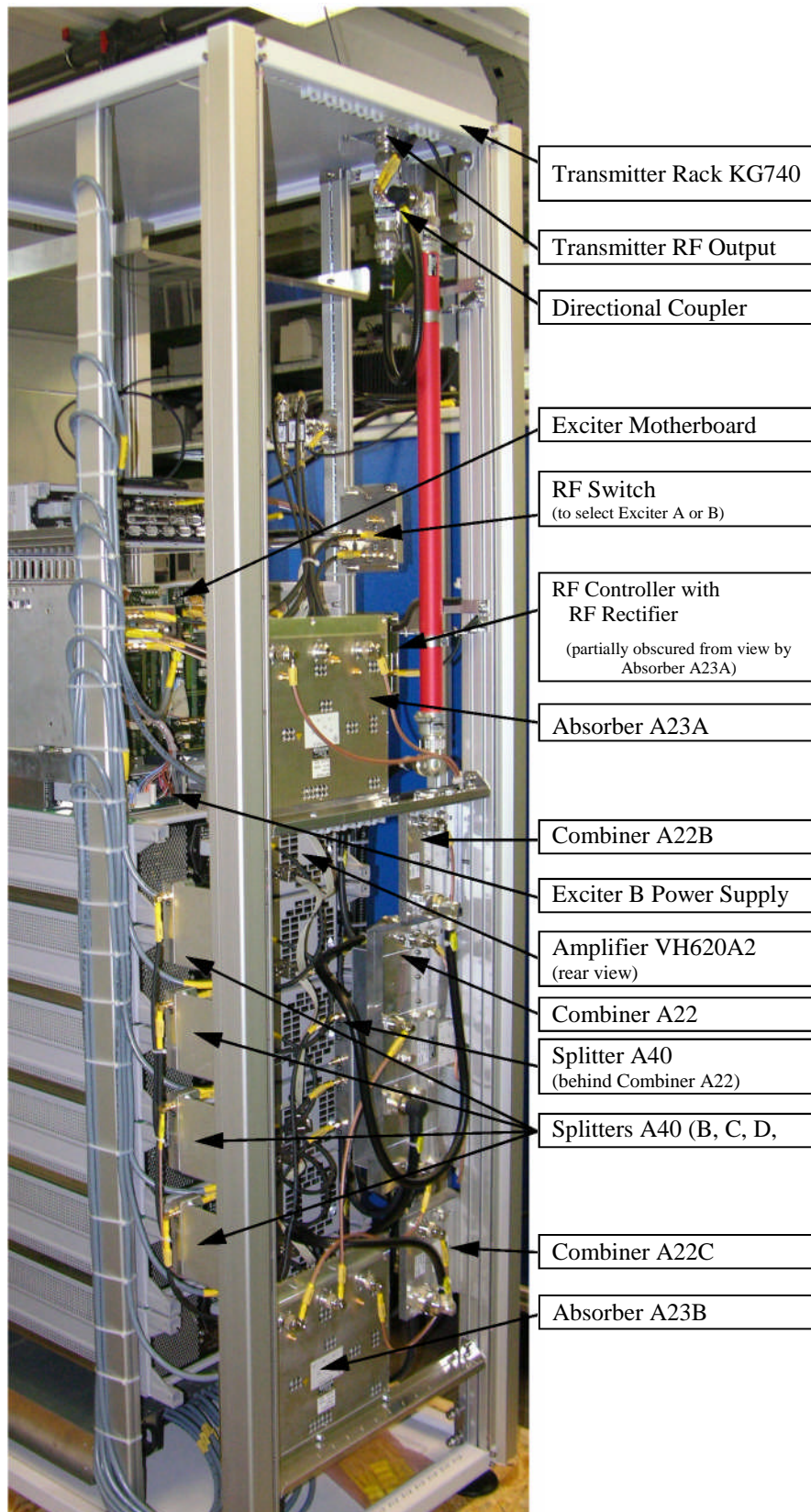
Rear View of SV7600 Transmitter with Side and Rear Cover Panels Removed
