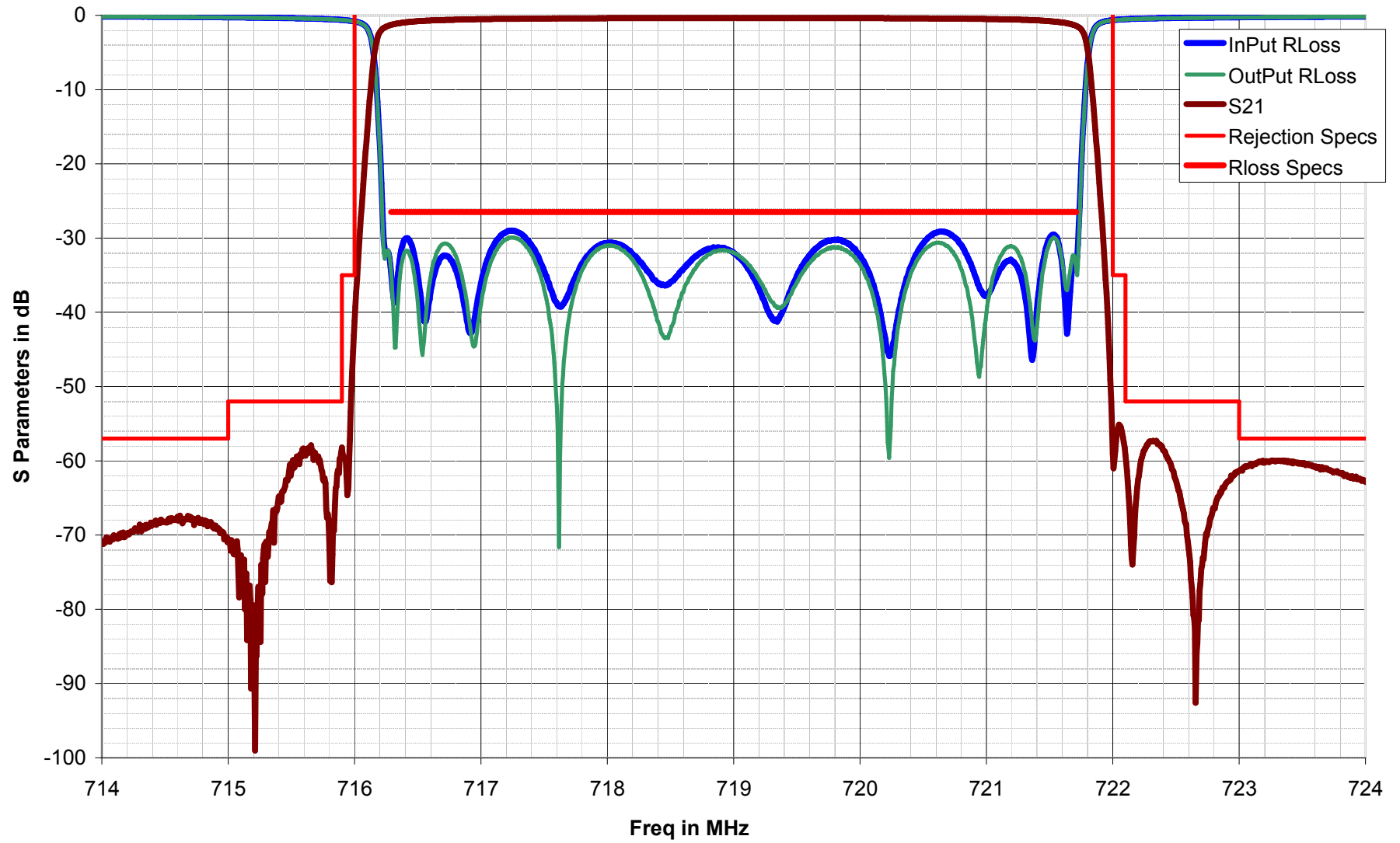
MFLO Filter S Parameters
