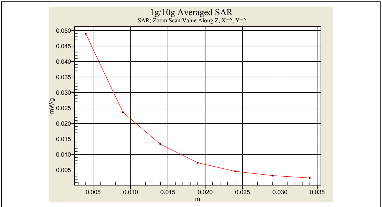
SAR Measurement _ Flat 802.11b CH1 (Tip_6MHz Data Rate)
