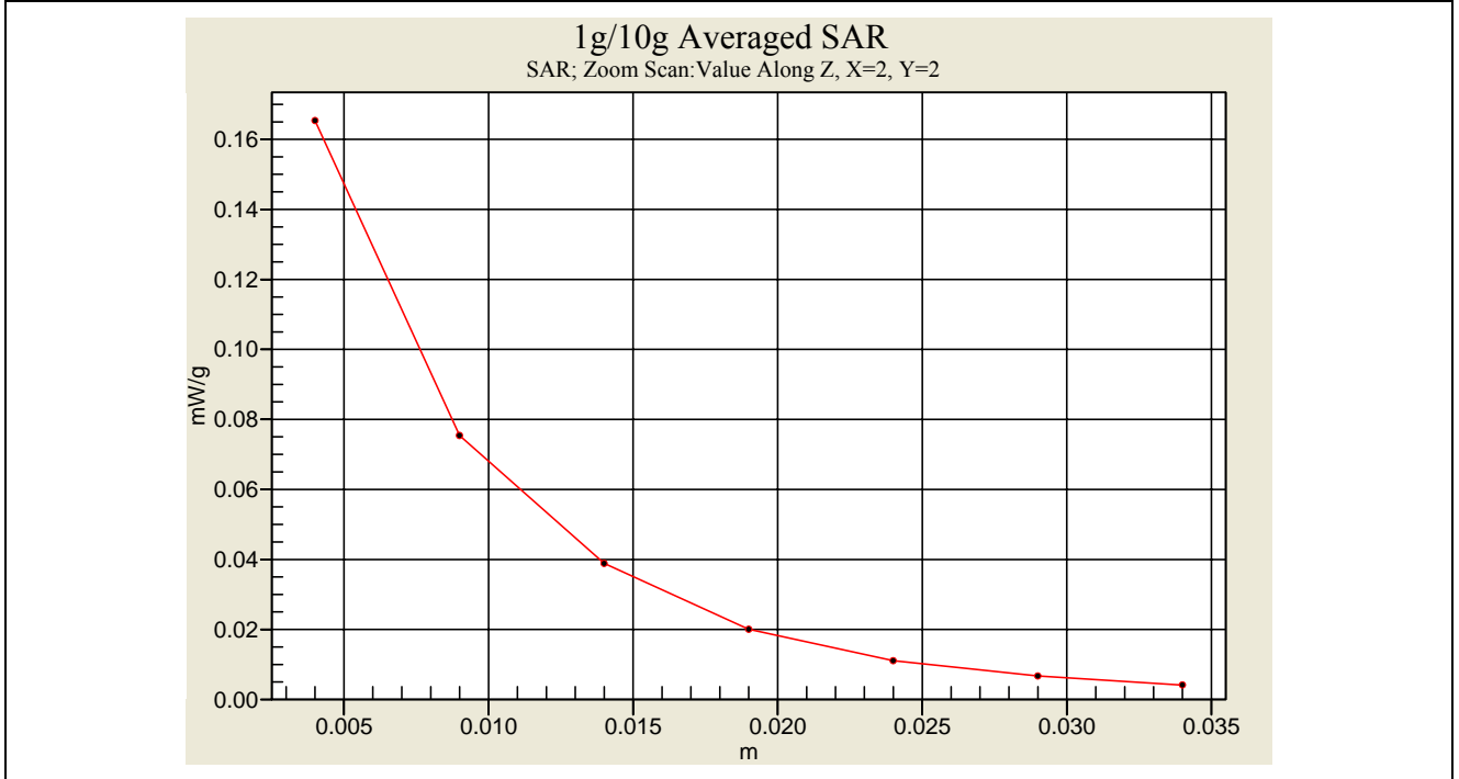
SAR Measurement _ Flat 802.11b CH1 (Tip_11MHz Data Rate)
