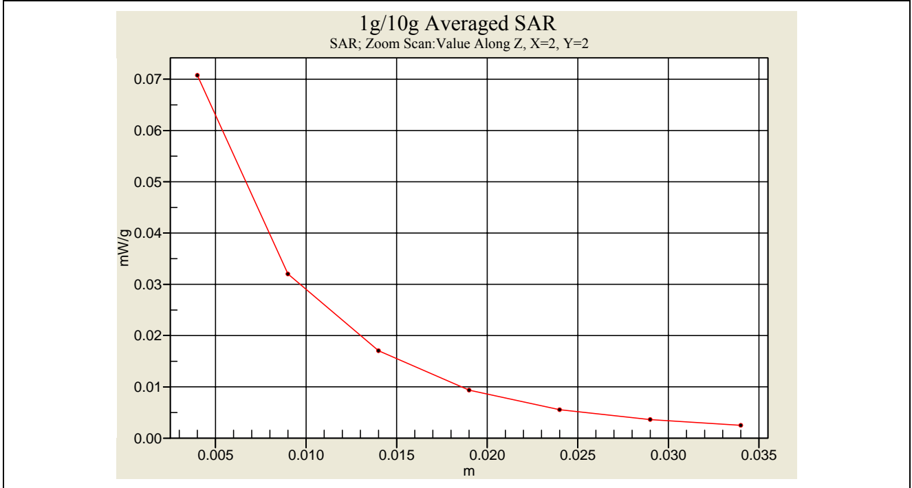
SAR Measurement _ Flat Cheek 802.11n CH1 (Tip_20MHz Bandwidth / 65MHz Data Rate)
