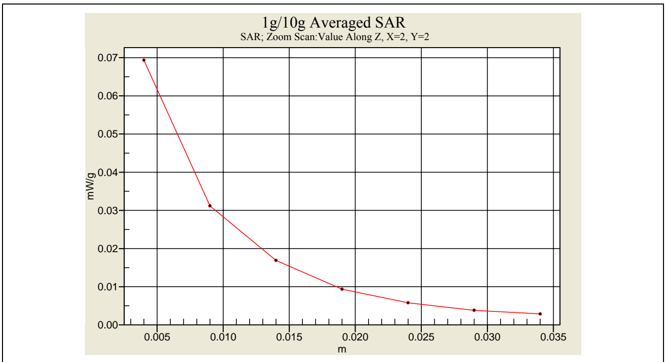
SAR Measurement _ Flat Cheek 802.11n CH3 (Tip_40MHz Bandwidth / 65MHz Data Rate)
