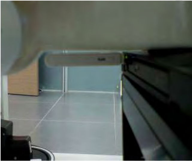
Fig.3 Back side of the EUT is paralleled with flat phantom, and spacing between EUT and Phantom is 4 mm.
