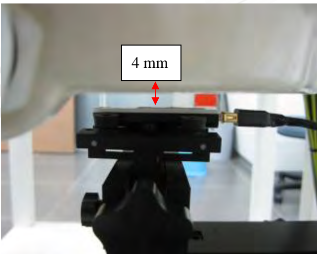
Fig.4 Front side of the EUT is paralleled with flat phantom, and spacing between EUT and Phantom is 4 mm.
