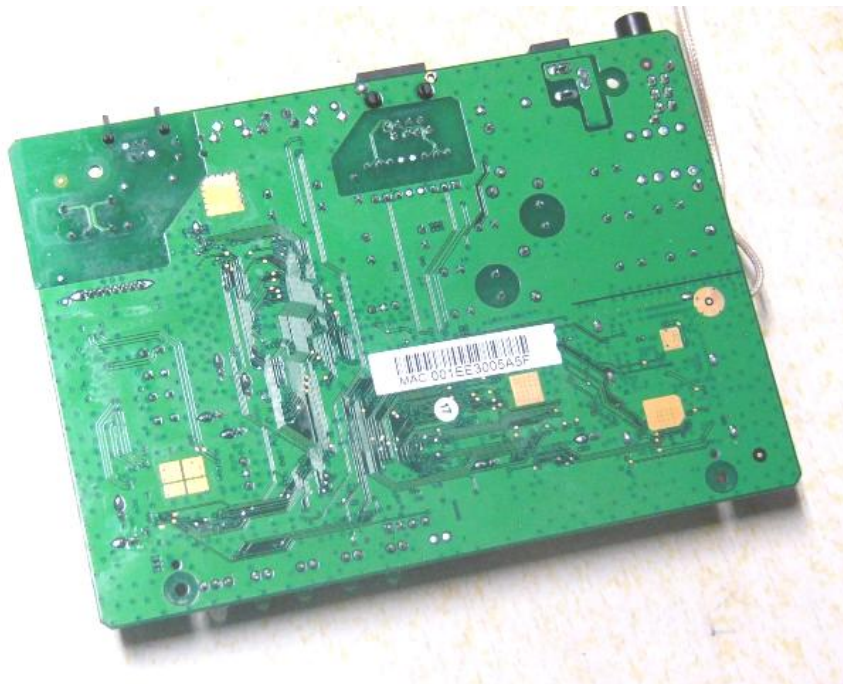
Main & RF board solder side
