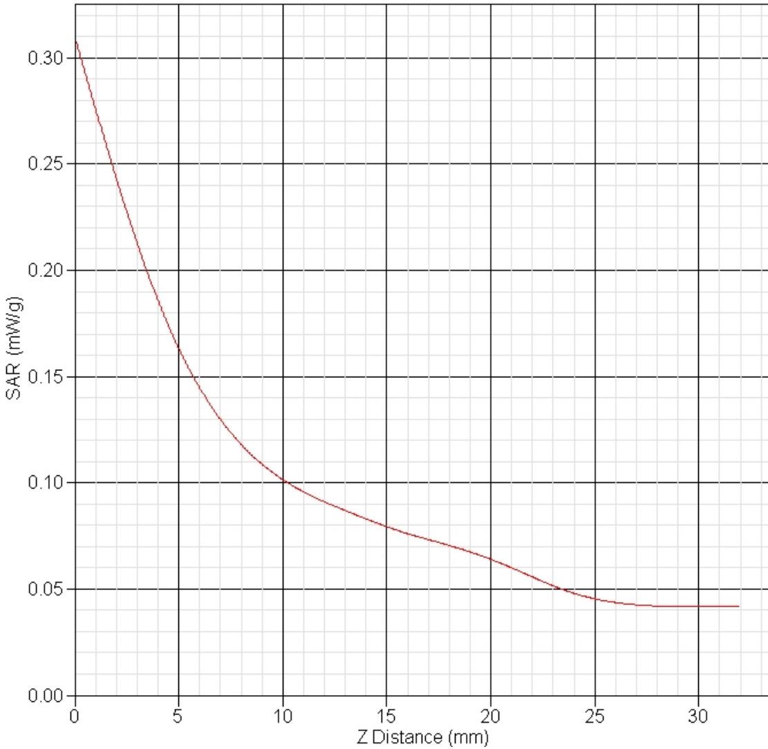
SAR-Z Axis
