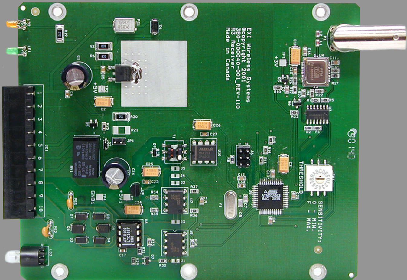
Receiver PCB Top View
