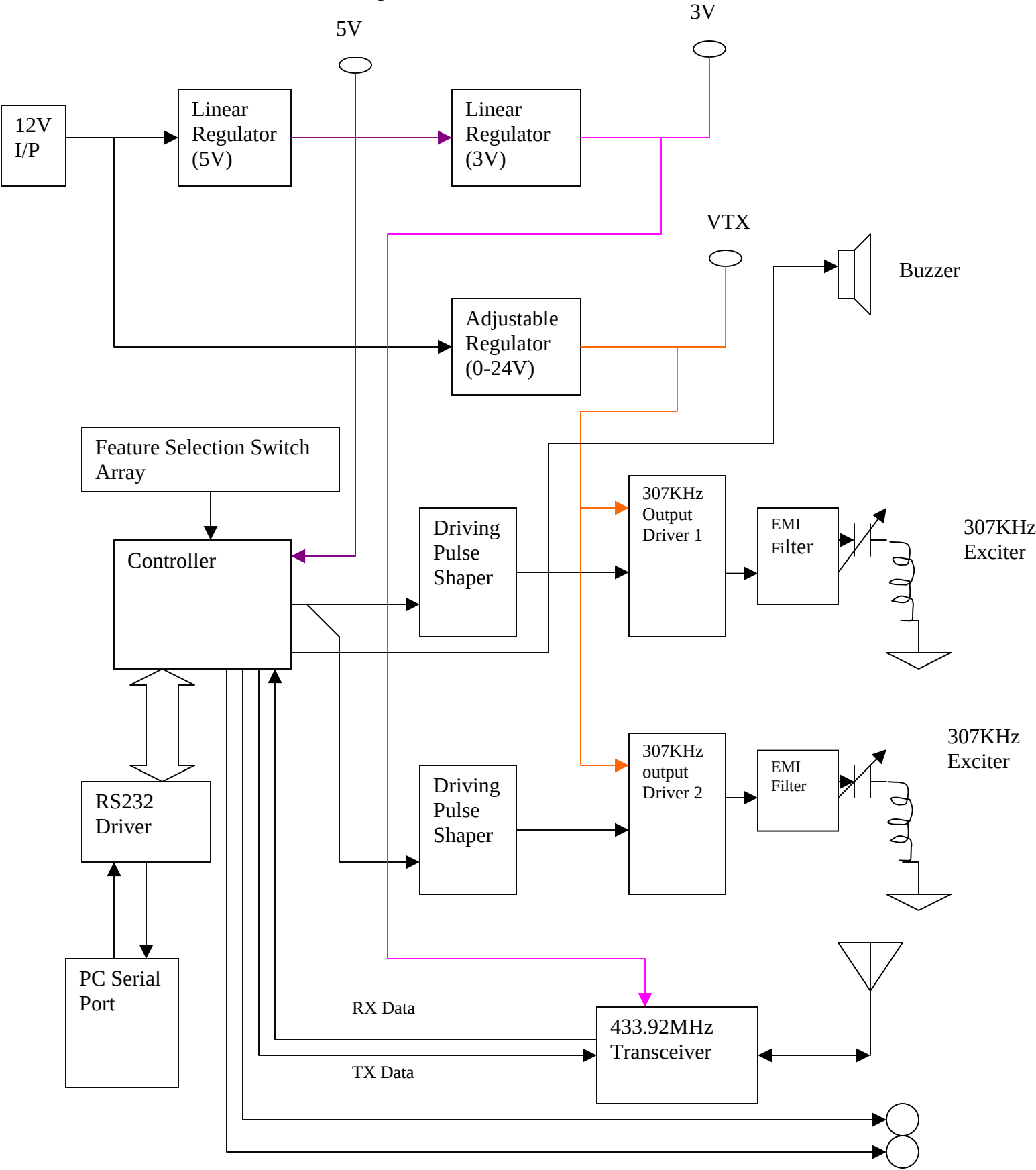
PTR Functional Block Diagram R1.10
