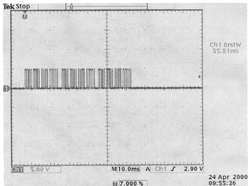
FIG 3.2 Decoded 433.92 MHz Off Body Message
