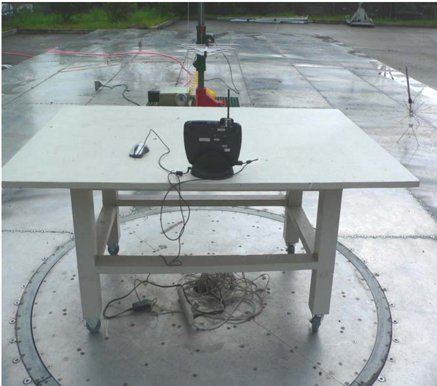
Radiated Emission Rear View
