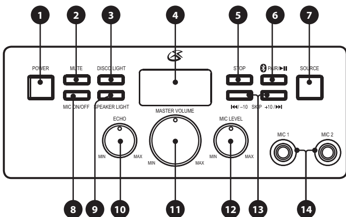
Front Controls
