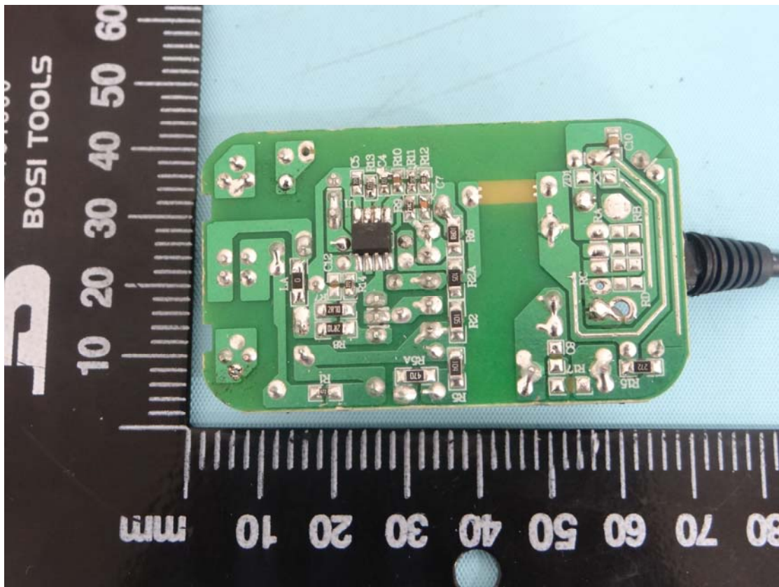
Adaptor (Model: FLD0710-9.0V0.6A-Z)
